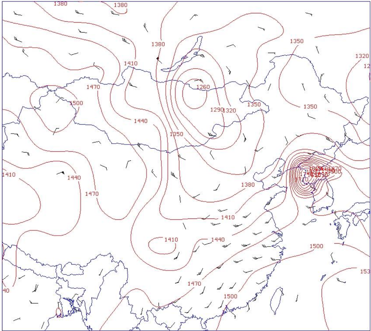
WIND(MPS) LEV=850 DAY=2011119 TIME=00 850MB Z(M) at 0 UTC on 29 Apr 2011
