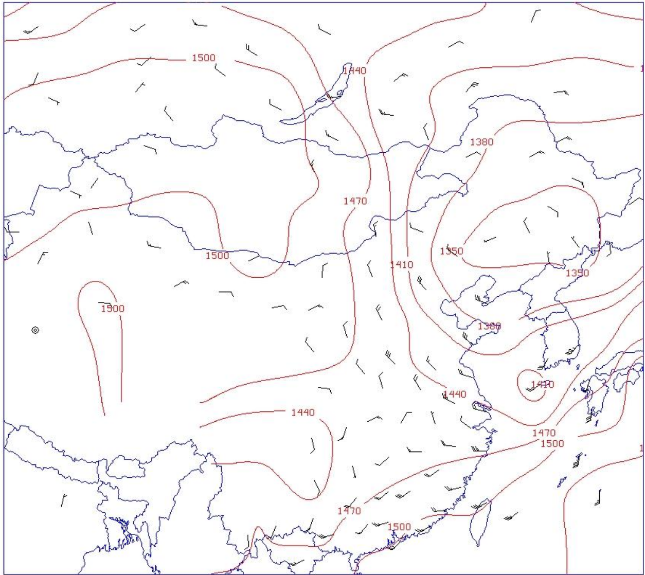
WIND(MPS) LEV=850 DAY=2011120 TIME=12 850MB Z(M) at 12 UTC on 30 Apr 2011
