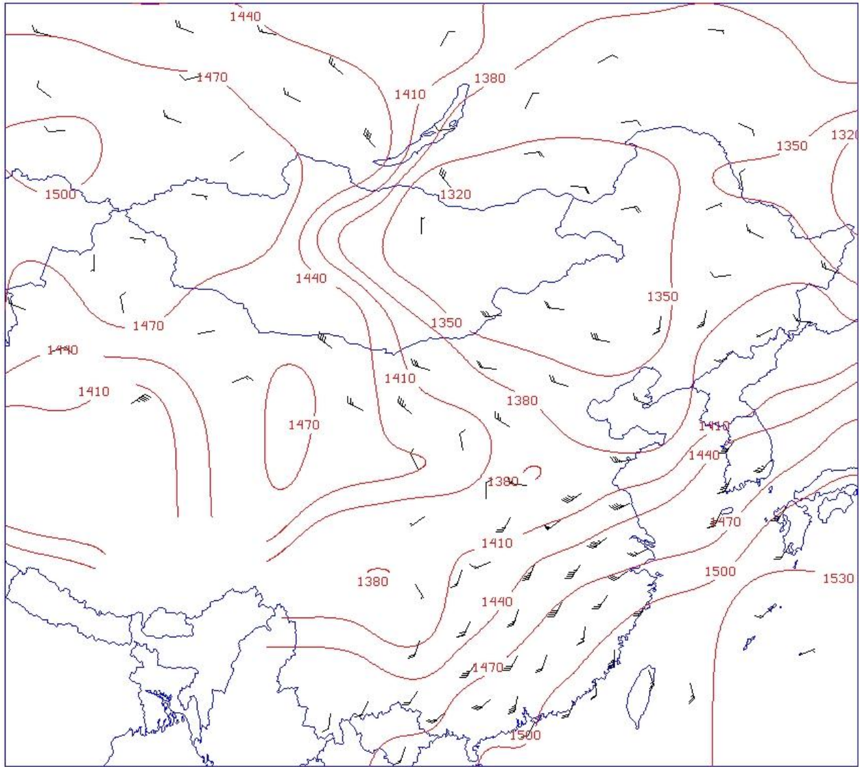
WIND(MPS) LEV=850 DAY=2011119 TIME=12 850MB Z(M) at 12 UTC on 29 Apr 2011
