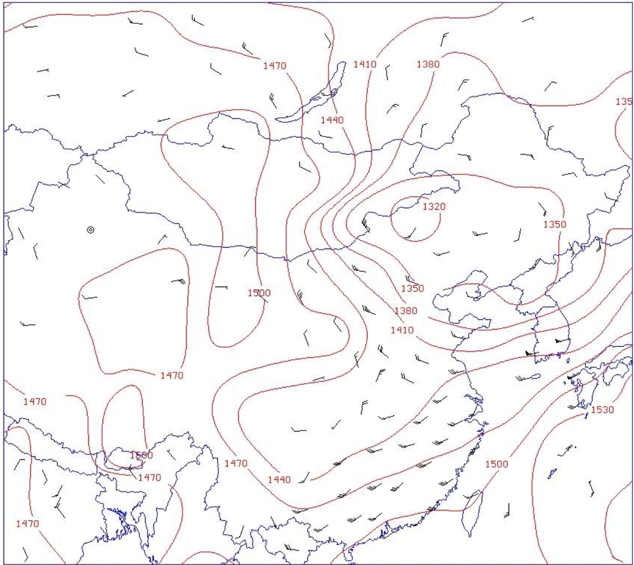
WIND(MPS) LEV=850 DAY=2011120 TIME=00 850MB Z(M) at 0 UTC on 30 Apr 2011
