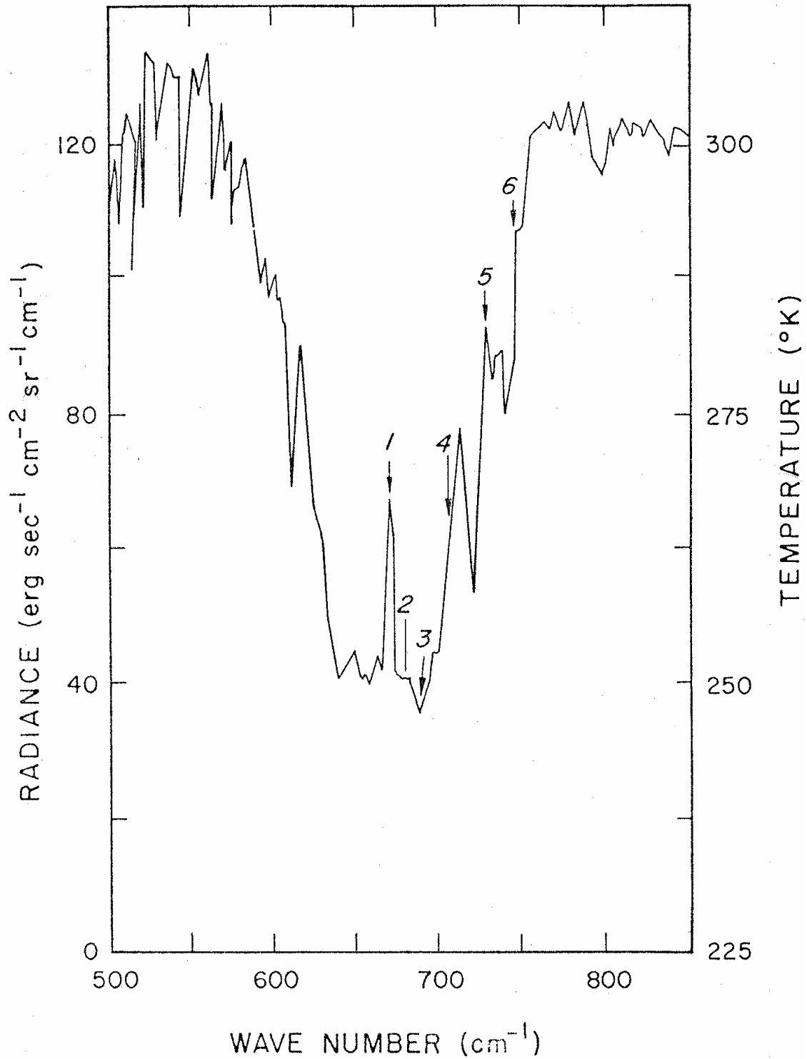
Figure 5.3: Outgoing radiance in terms of black body temperature in the vicinity of 15\mu\text{m} \text{CO}_2 band observed by the IRIS on Nimbus IV. The arrows denote the spectral regions sampled by the VTPR instrument.
