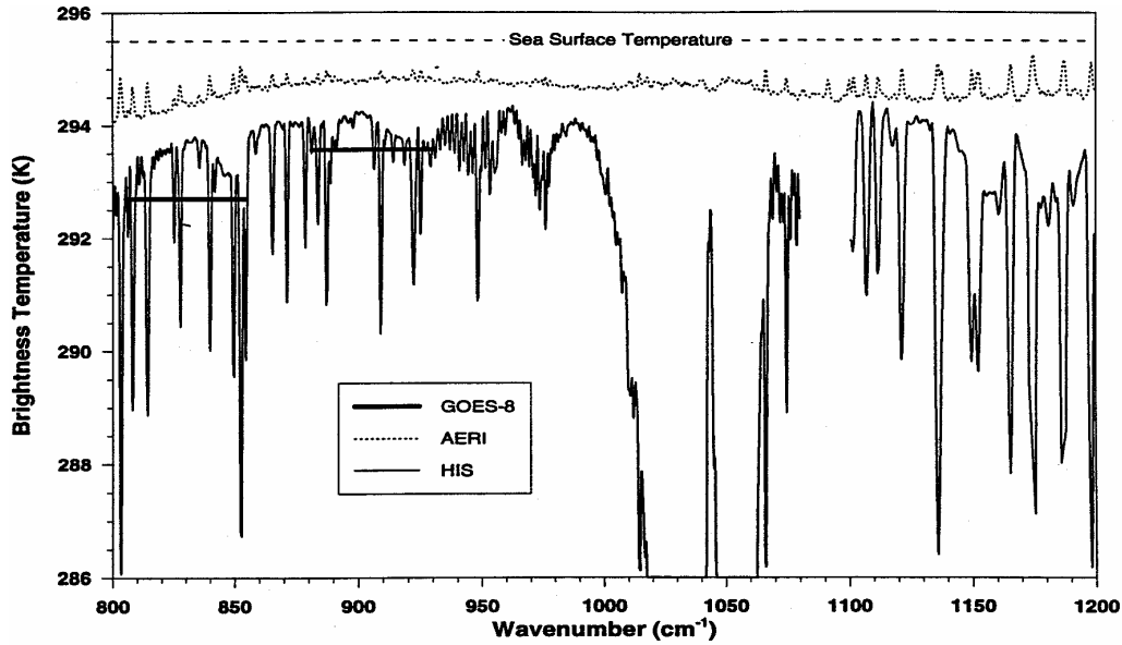
Figure 7.4: Comparison of ocean brightness temperatures measured by a ship borne interferometer (AERI), by an interferometer (HIS) on an aircraft at 20 km altitude, and the geostationary sounder (GOES-8). Corrections for atmospheric absorption of moisture, non-unit emissivity of the sea surface, and reflection of the atmospheric radiance from the sea surface have not been made.
