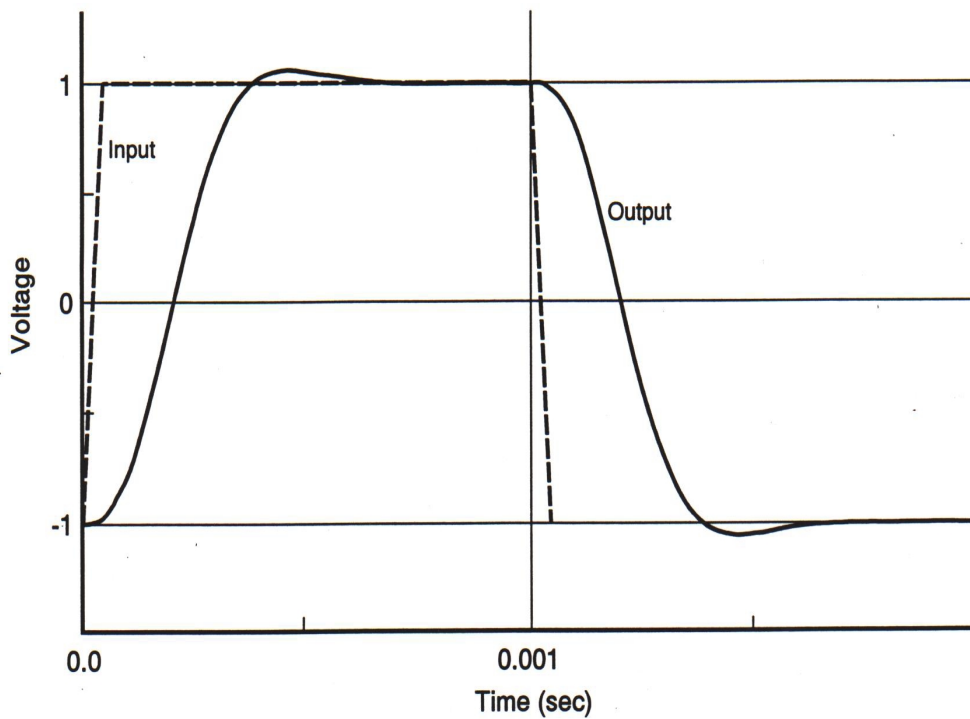
Figure 12.4: The step response function for GOES-8.
