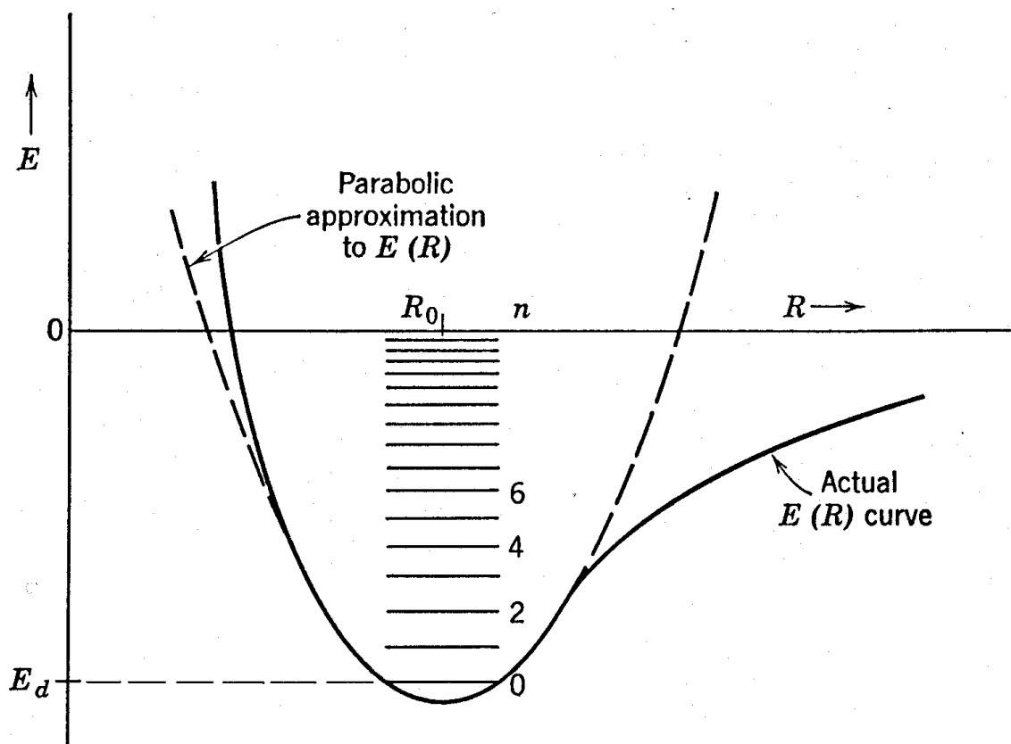
Figure 3.2: Vibrational energy levels of a diatomic molecule.
