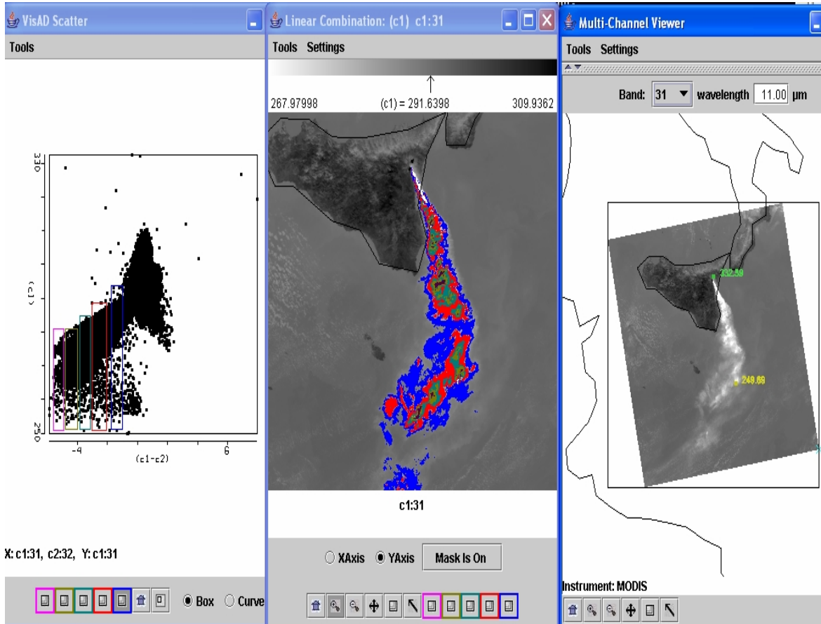
Figure 21: (right) Infrared window image of [band 31 (11 \mu m)] of Mt Etna eruption on 28 Oct 2002; (middle) color enhanced image of [band 31 (11 \mu m) - band 32 (12 \mu m)] with blue, red, green, olive, and purple indicating progressively larger BT differences from 0 to -6 C; and (left) scatter plot of [band 31 (11 \mu m) - band 32 (12 \mu m)] on the x-axis and band 31 (11 \mu m) on the y-axis. The larger differences come from the denser ash.
