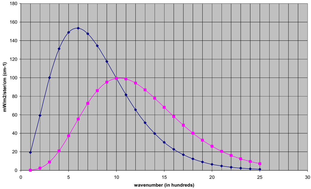
Figure 2.4: Planck radiance curves at 300 K. Wavenumber are given in units of 100 cm -1 ; the corresponding wavelengths in cm are determined from the reciprocal of the wavenumber. Purple boxes show B(\lambda, T) in units of mW/ster/m 2 /cm (per unit wavelength) and blue diamonds show B(\nu, T) in units of mW/ster/m 2 /cm -1 (per unit wavenumber). B(\lambda, T) is shown multiplied by a factor of 10^{-6} (e.g. B(10 \mu\text{m}, 300 \text{ K}) is 9.9 \times 10^7 ) while B(\nu, T) is shown multiplied by a factor of 1 (e.g. B(1000 \text{ cm}^{-1}, 300 \text{ K}) is 99.0). Note that Wiens law for B(\nu, T) becomes \nu(\text{max}) = 1.95T \text{ (cm}^{-1}\text{)} while the more familiar form for B(\lambda, T) is \lambda(\text{max}) = .2897/T \text{ (cm)} .
