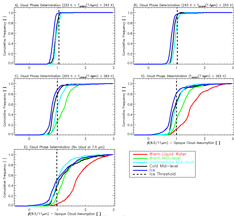
Figure 9: The cumulative distribution function (CDF) of \beta_{\text{opaque}}(8.5/11\mu\text{m}) for 5 CALIOP-derived cloud top temperature bins is shown for 5 different bins of 7.4\mu\text{m} opaque cloud temperature ( T_{\text{opaque}}(7.4\mu\text{m}) ). In panel A, 233\text{ K} < T_{\text{opaque}}(7.4\mu\text{m}) < 243\text{ K} . In panel B, 243\text{ K} < T_{\text{opaque}}(7.4\mu\text{m}) < 253\text{ K} . In panel C, 253\text{ K} < T_{\text{opaque}}(7.4\mu\text{m}) < 263\text{ K} . In panel D, T_{\text{opaque}}(7.4\mu\text{m}) > 263\text{ K} . Finally in panel E, T_{\text{opaque}}(7.4\mu\text{m}) is undefined because the cloud is well below the peak of the 7.4\mu\text{m} weighting function or the cloud is too optically thin to be differentiated from the 7.4\mu\text{m} clear sky signal.
