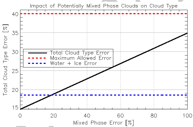
Figure 19: Same as Figure 18, except for cloud type.
