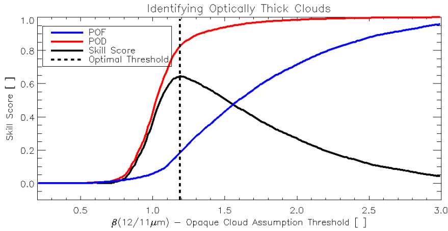
Figure 6: Peirce-Hanssen-Kuipers skill score metrics are shown as a function of the \beta_{\text{sopaque}}(12/11\mu\text{m}) threshold used to distinguish between clouds with a 11\text{-}\mu\text{m} cloud optical depth of less than and greater than 2.0. The probability of false alarm (POF) is shown in blue, the probability of detection (POD) is shown in red, and the skill score is depicted by the black solid line. The \beta_{\text{sopaque}}(12/11\mu\text{m}) threshold that maximizes the skill score is depicted by the dashed black line. This analysis is based on over 8000 SEVIRI/CALIOP match-ups.
