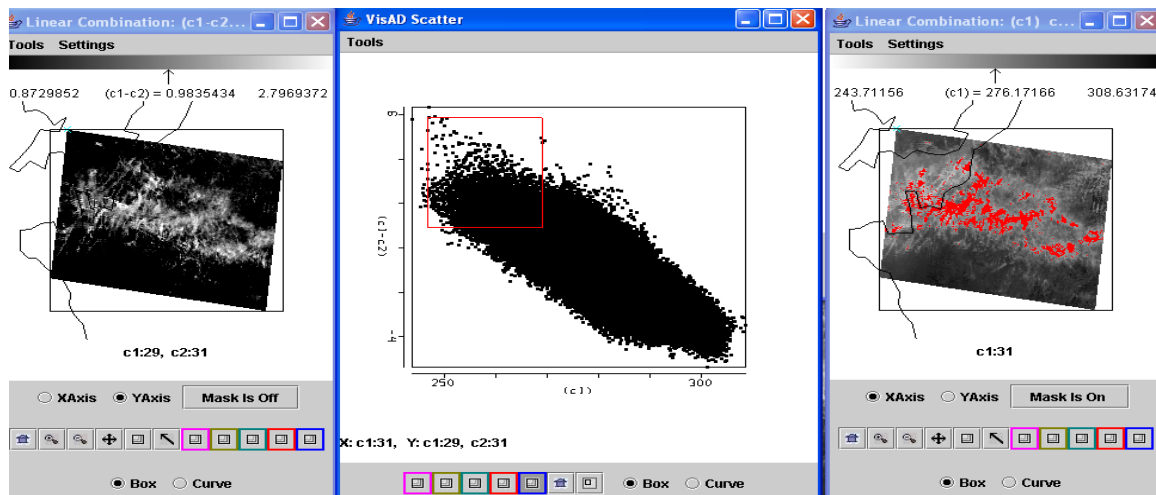
Figure 5a: Scatter plot of BT8.6-BT11 (left image) versus BT11 (right image) with \text{BT8.6-BT11} > 1 and \text{BT11} > 270 highlighted in red.
