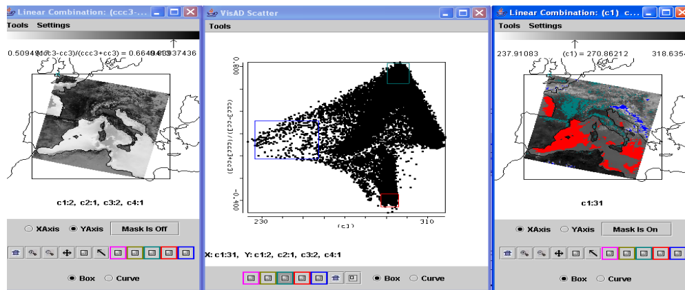
Figure 2: Scatter plot of NDVI (left image & y-axis) versus BT11 (right image & x-axis)
