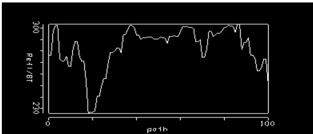
Figure 15.12: Brightness temperatures in Band 31 (LIRW, 11 micron) from the Alps, over the Adriatic Sea, through northern Italy, and into the Tyrranean Sea. Cloud band has BT of 230 K.
