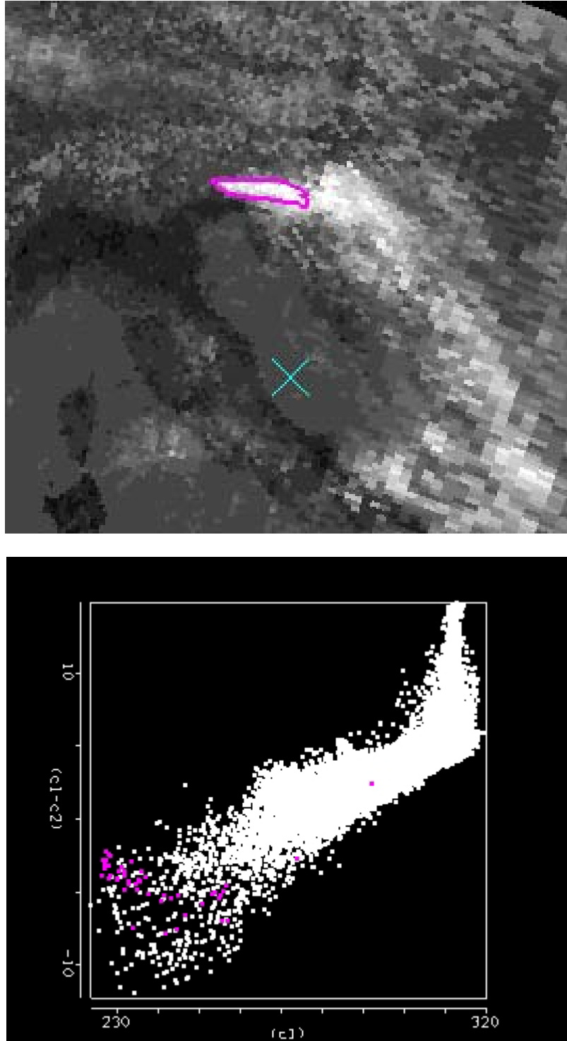
Figure 15.14: Scatter plot (bottom) of [BT31 (11 \mu\text{m} )] on the x-axis and [BT31 (11 \mu\text{m} ) – BT29 (8.5 \mu\text{m} )] on the y-axis. Ice cloud in BT31 image (top) shows negative [BT31-BT29] values in scatter plot.
