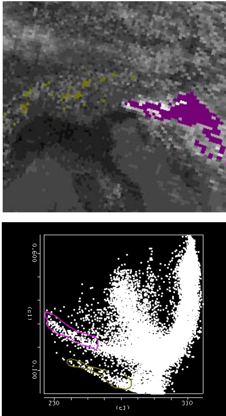
Figure 15.16: Scatter plot (bottom) of reflectance in 1.6 \mu\text{m} (band 6) versus brightness temperature in 11 \mu\text{m} (band 31). BT(31) image (top) shows snow in Alps (green) is distinguished from ice in clouds (purple) by differing band 6 reflectances.
