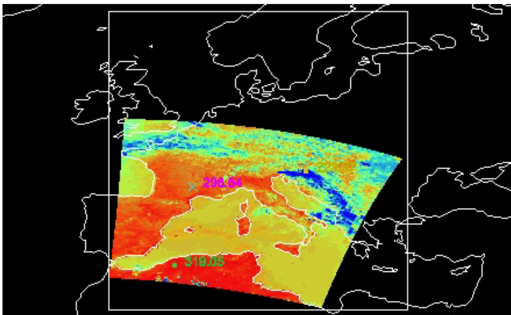
Figure 15.10: MODIS IRW (Band 31) brightness temperature image displayed with a color scale range from 240 K (blue) to 320 K (red).
