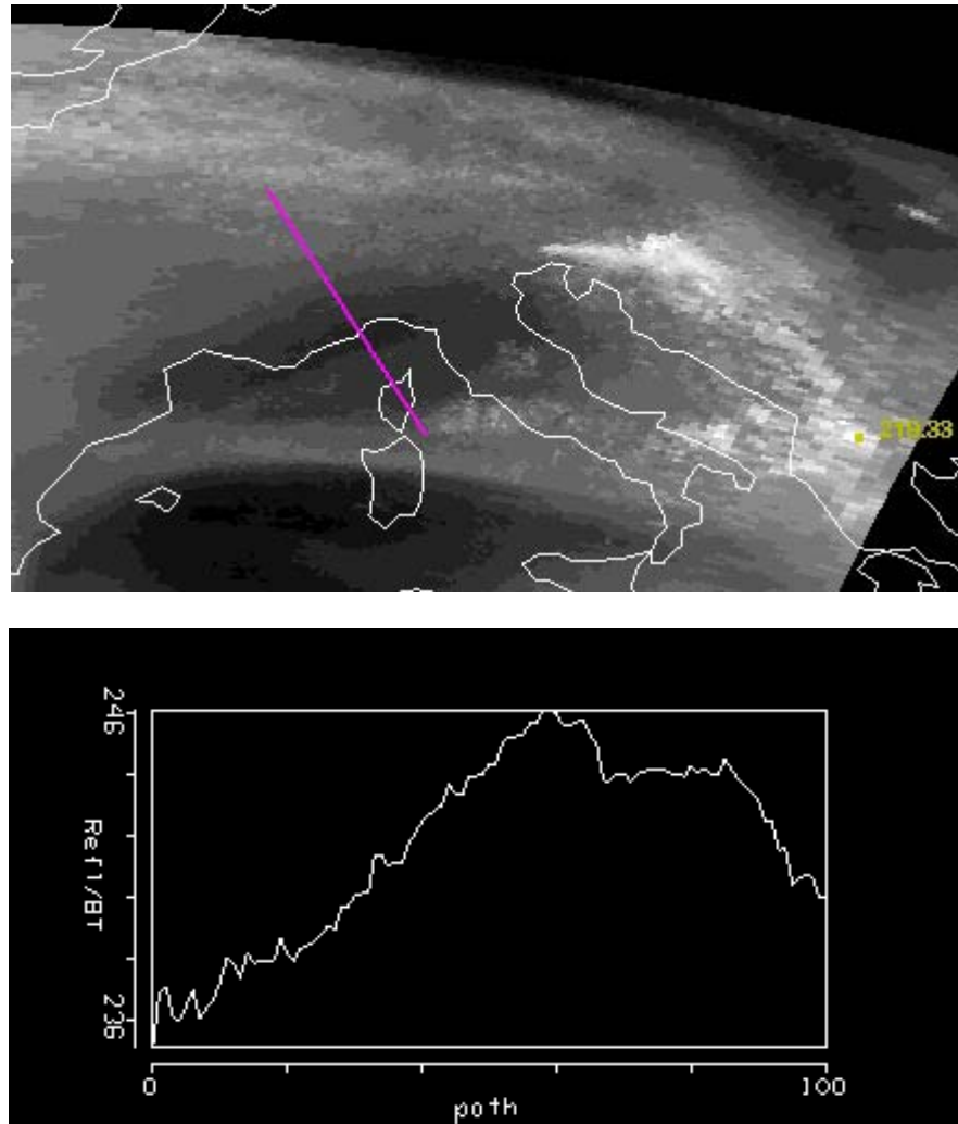
Figure 15.15: Cross-section plot (bottom) of BT(H 2 O) for the 6.7 \mu\text{m} (band 27) water vapor sensitive band (image on top) from north to south over a dry slot. The dry slot is about 10 C warmer than the neighboring wet areas.
