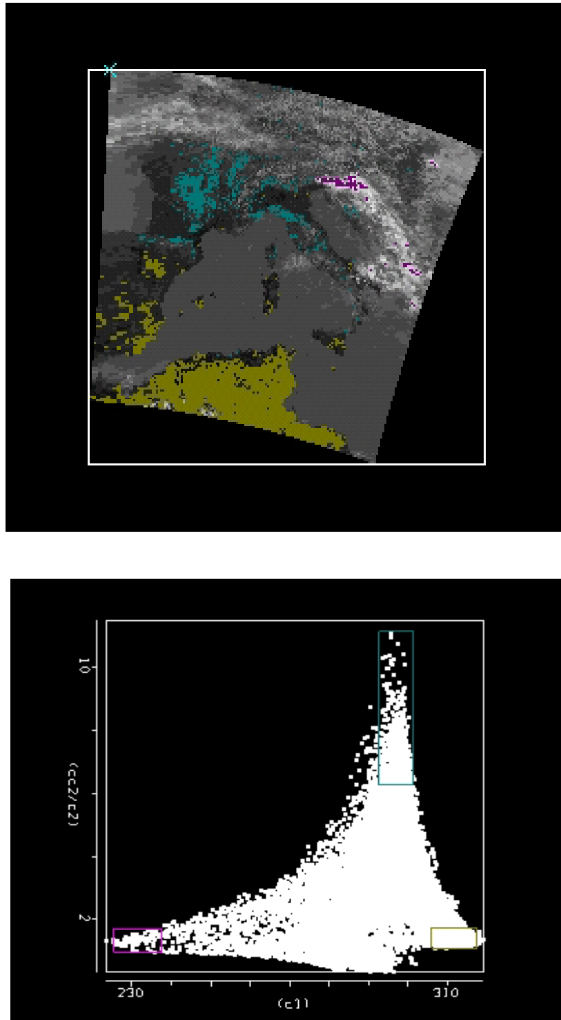
Figure 15.17: Scatter plot (bottom) of brightness temperature in 11\ \mu\text{m} (band 31) vs reflectance ratio 0.8/0.6\ \mu\text{m} (band 2 / band 1). BT(31) image (top) shows clouds (purple with b2/b1 close to one and BT31 cold), non-vegetated land (green with b2/b1 close to one and BT31 hot), and vegetated land (blue with b2/b1 much greater than one and BT31 warm).
