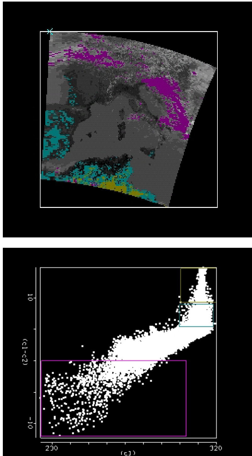
Figure 15.13: Scatter plot (bottom) of [BT31 (11 \mu\text{m} )] on the x-axis and [BT31 (11 \mu\text{m} ) – BT29 (8.5 \mu\text{m} )] on the y-axis. Large negative [BT31-BT29] indicates ice cloud in BT31 image (top).
