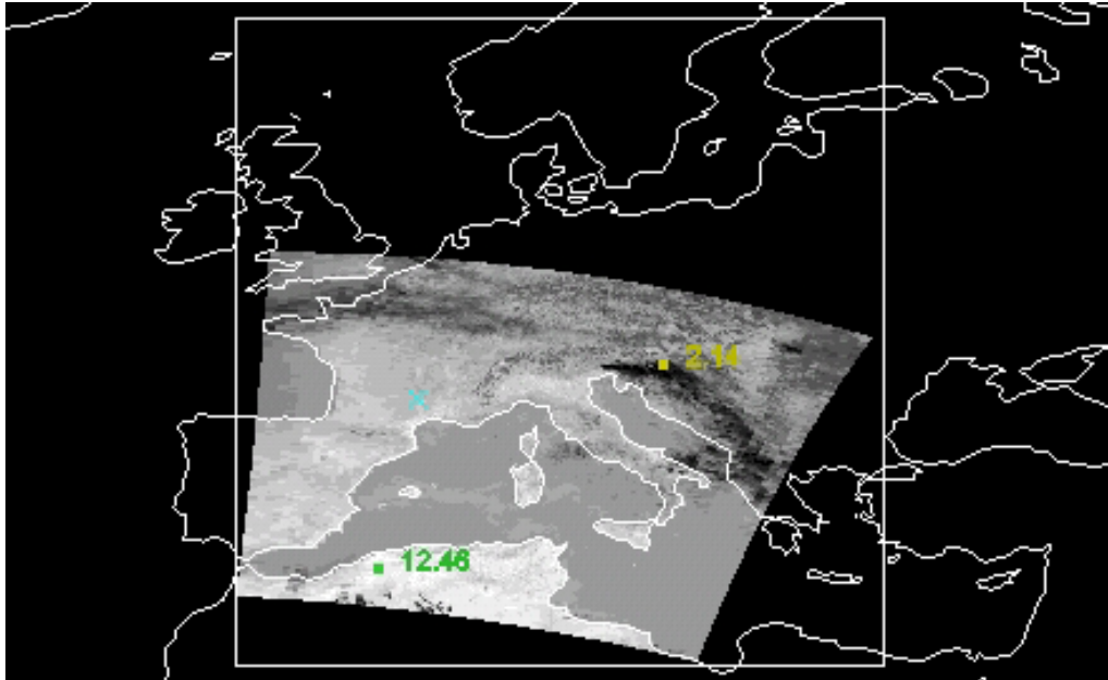
Figure 15.9: MODIS Display (in hydra) of MODIS IRW (Band 31) radiances ( W/m^2/micron/ster ) with minimum 2.14 and maximum 12.46 values the tool bar indicated on the screen.
