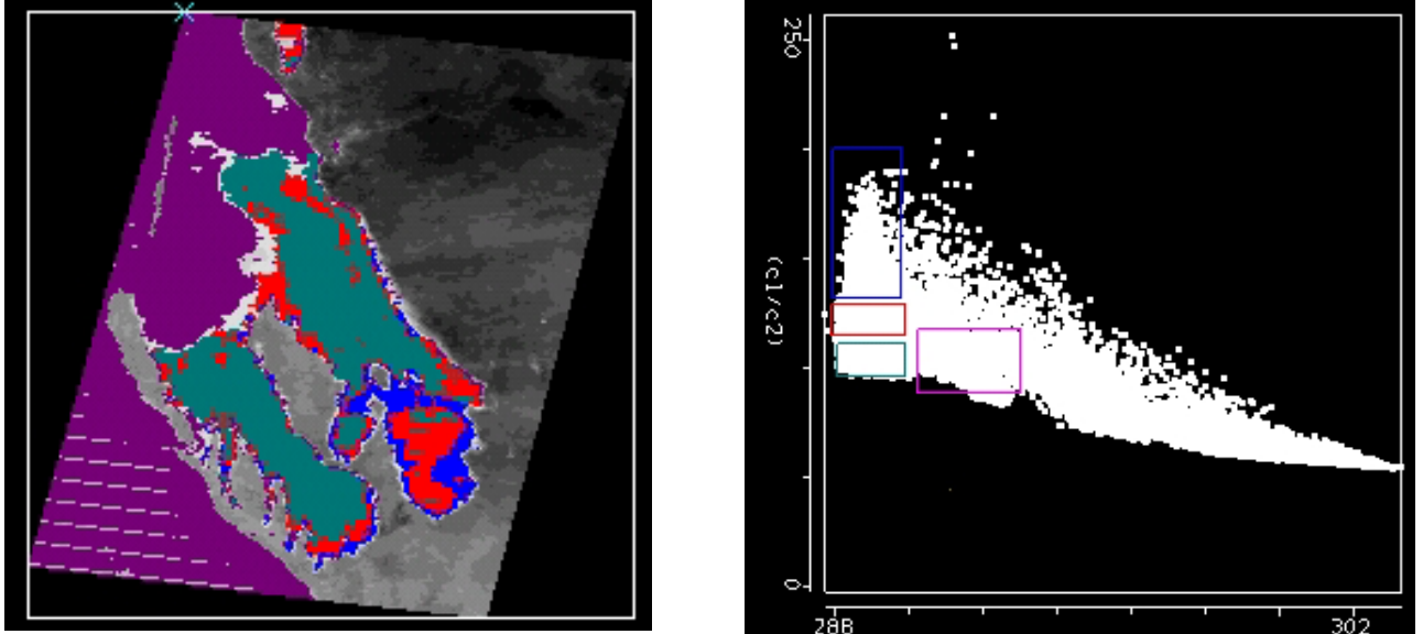
Figure 15.22: (left) Image of infrared window brightness temperature (indicative of sea surface temperature) showing waters within Shark Bay (blue, red, green) are about 3 C cooler than the Leeuwin current waters (purple) along the WA coastline. (right) Scatter plot over Shark Bay of band 31 ( 11\mu\text{m} ) on the x-axis and band 9 ( 0.44\mu\text{m} ) / band 12 ( 0.57\mu\text{m} ) on the y-axis. Low ratio values are an indication of chlorophyll concentrations.
