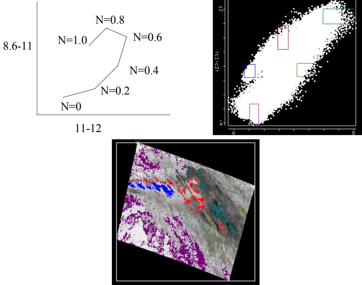
Figure 15.19: (top left) diagram of [BT(8.6)-BT(11)] versus [BT(11)-BT(12)] as a function of cloud fraction; (top right) scatter plot of [BT(8.6)-BT(11)] versus [BT(11)-BT(12)] for cloud scene on 29 May 2001, (bottom) subsets of scatter plot colored onto image of [BT(11)-BT(12)] demonstrating concept of top diagram.
