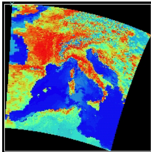
Figure 15.20: A pseudo image of normalized vegetation index [\text{band 2 (0.86}\mu\text{m)} - \text{band 1 (0.65}\mu\text{m)}] / [\text{band 2 (0.86}\mu\text{m)} - \text{band 1 (0.65}\mu\text{m)}] . Regions with some vegetation are clearly distinguished from those with little. Dry desert-like regions on the heel of Italy and in northern Africa show vegetation indices below 0.3; fertile valleys in northern Italy show indices above 0.8.
