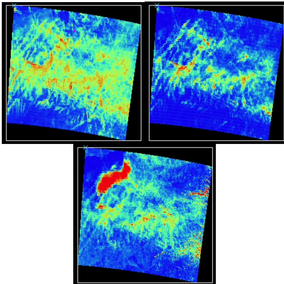
Figure 15.18: Contrails seen in (top left) positive values of [\text{BT}(8.6) - \text{BT}(11)] in yellow and red, (top right) high reflectance in [r(1.38)] , and (bottom) high reflectance in [r(0.6)] . Some of the contrails are not seen in the visible.
