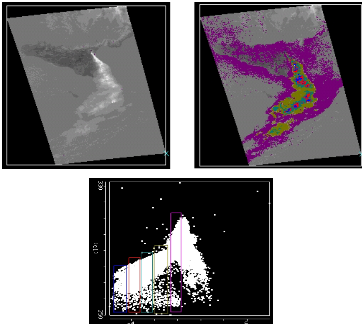
Figure 21: (top left) Infrared window image of [band 31 ( 11\mu\text{m} )] of Mt Etna eruption on 28 Oct 2002; (top right) color enhanced image of [band 31 ( 11\mu\text{m} ) - band 32 ( 12\mu\text{m} )] with purple, olive, green red, and blue indicating progressively larger BT differences from 0 to -6\text{ C} ; and (bottom) scatter plot of [band 31 ( 11\mu\text{m} ) - band 32 ( 12\mu\text{m} )] on the x-axis and band 31 ( 11\mu\text{m} ) on the y-axis. The larger differences come from the denser ash.
