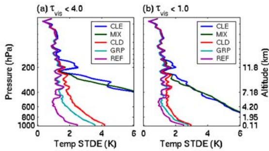
Figure 1. Retrieval accuracy analyses through semi-transparent clouds: (a) for optical depth ( \tau_{\text{vis}} ) less than 4, (b) for optical depth ( \tau_{\text{vis}} ) less than one.
