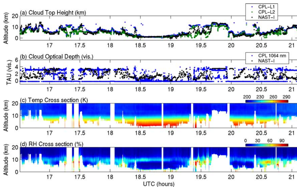
Figure 2. Panel (a) NAST-I retrieved cloud top height compared with the CPL measured cloud top heights of the top 2 layers (L1 and L2). Panel (b) NAST-I retrieved cloud optical depth (effective visible) compared with the CPL measurement. Panels (c) and (d) plot NAST-I retrieved temperature and relative humidity vertical cross sections, respectively. The areas wiped off are under the top layer clouds where the cloud visible optical depth is larger than one and under the lower “opaque” cloud.
