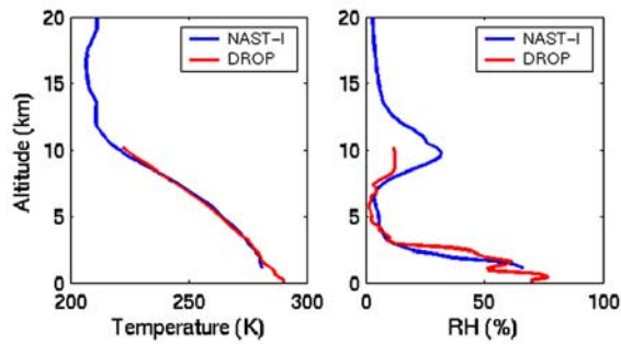
Figure 3. Profile comparison between the mean of NAST-I retrievals and coincident dropsondes.
