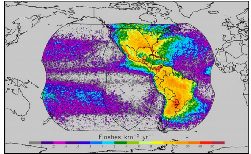
LIS/OTD Combined Lightning 1997-2005
