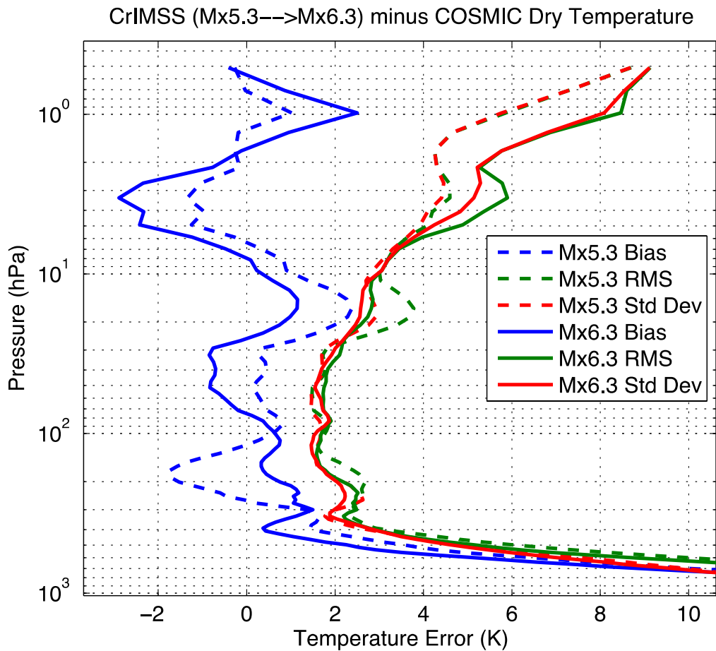
Figure 17.3.1. Impact on the AVTP bias (blue), RMS (green), and standard deviation (red) of the official CrIMSS IDPS product relative to coincident matchups from the COSMIC GPS RO network from the change in IDPS version Mx5.3 (dashed) to Mx6.3 (solid). The bias and RMS are considerably improved in the 30 mb to 300 mb range for which the COSMIC GPS RO is most accurate.
