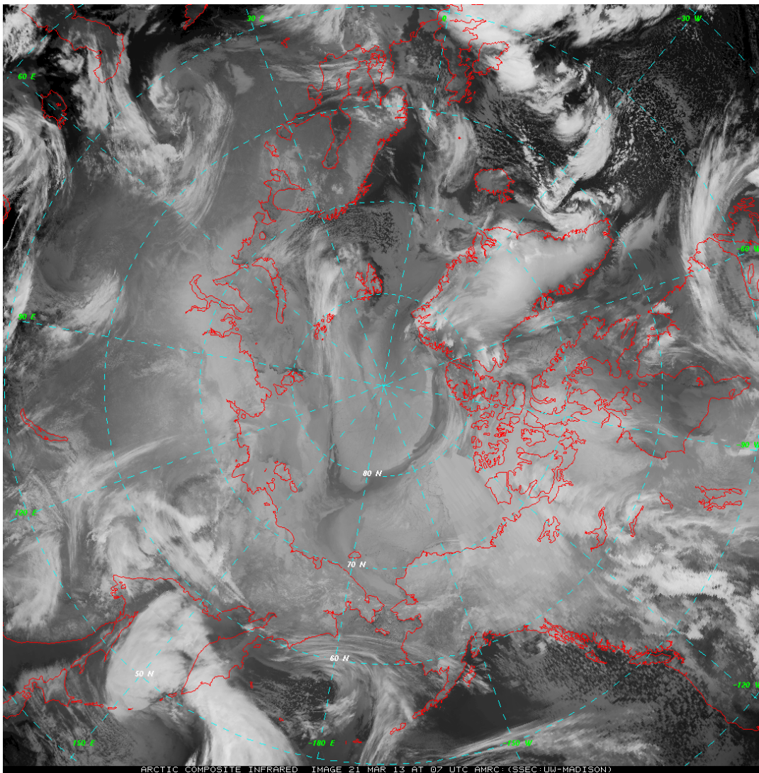
Figure 4.3.1. An example Arctic composite infrared image from 21 March 2013 at 7 UTC depicting the good coverage possible over the entire Arctic basin from the mosaic of polar orbiting and geostationary satellite observation.
