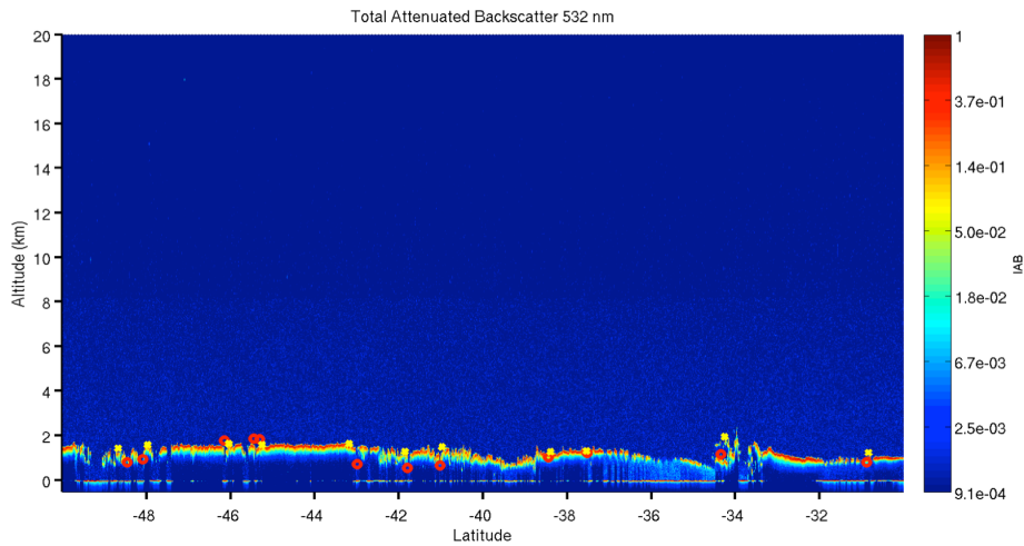
Figure 8.5.4. CALIPSO total attenuated backscatter with collocated AMV-estimated cloud height plotted in red, and CALIPSO-estimated cloud tops in yellow. AMV height assignment shows good agreement with low-level water clouds.
