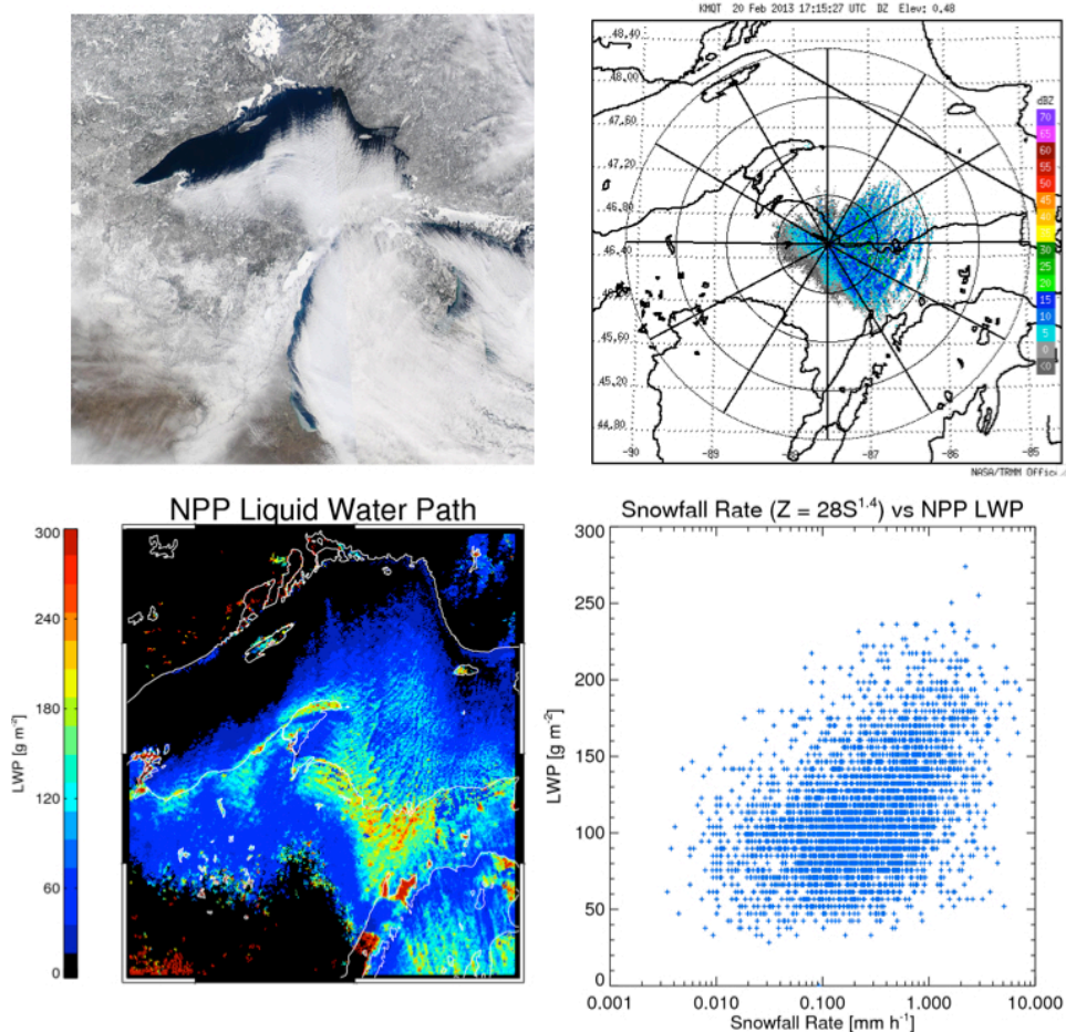
Figure 3.6.2. Aqua MODIS true color composite image (top left), KMQT NEXRAD base scan radar reflectivity (dBZ) at 1715 UTC (top right), Suomi NPP AWG cloud LWP ( \text{g m}^{-2} ) (bottom left) near 1715 UTC, and NEXRAD-derived snowfall rate ( \text{mm h}^{-1} ) versus LWP for 1715 UTC 20 Feb 2013.
