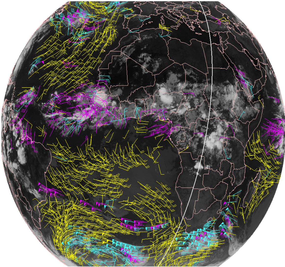
Figure 8.8.1. IRW AMVs from Meteosat-9 plotted with the CALIPSO transect locations in white.
