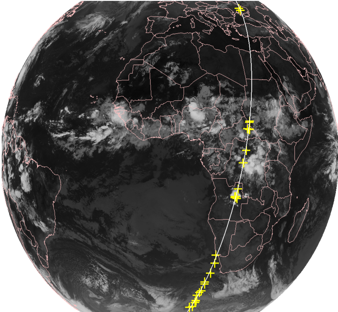
Figure 8.8.2. AMV and CALIPSO match locations (yellow pluses) for 15 Sept. 2011, at 00 UTC.
