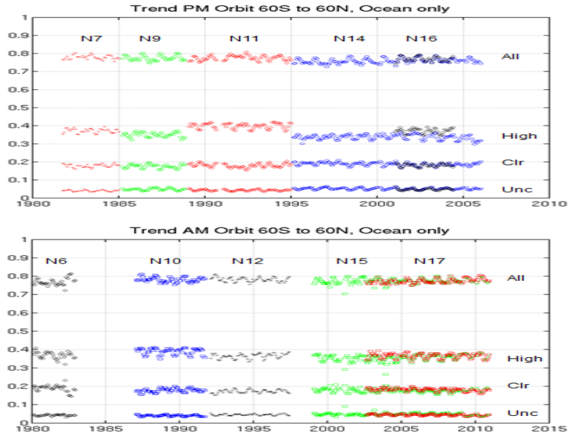
Figure 36.3. Afternoon and morning high (CTP<440 hPa) cloud over ocean trends from 1980 through 2009 given in fraction of total HIRS observations after the spectral shifts.
