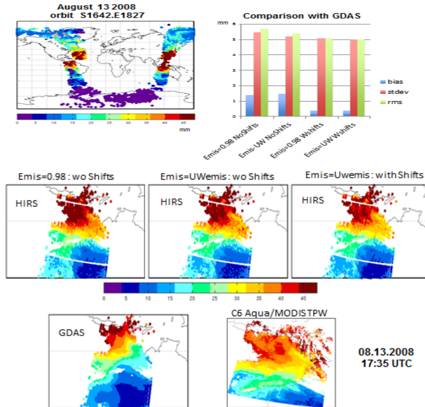
Figure 36.4. NOAA18/HIRS TPW compared to GDAS and Aqua/MODIS TPW.
