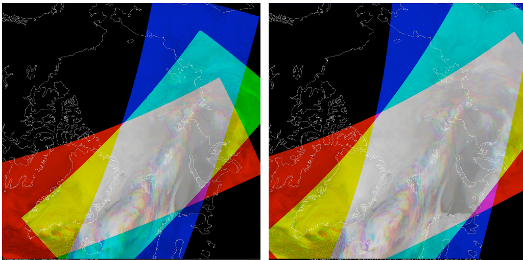
Figure 4.2.2.2. The gray region represents the overlap in three orbits where the polar winds are derived for MODIS (left) and VIIRS (right).
