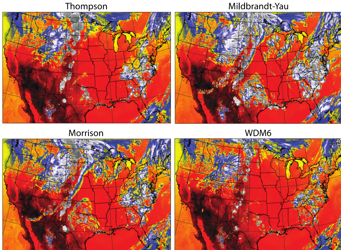
Figure 9.9.1. Simulated GOES-13 10.7 mm brightness temperatures (K) valid at 2200 UTC on 22 May 2012 for four of the CAPS ensemble members.
