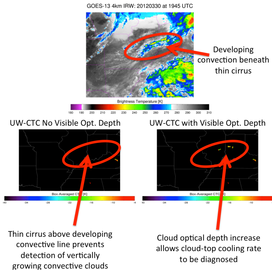
Figure 3.1.1. Top panel is GOES-13 11 \mu\text{m} brightness temperature valid at 1945 UTC 30 March 2012; developing convection beneath thin cirrus clouds is highlighted over eastern Illinois and central Indiana. Bottom left panel is UW-CTC output without visible optical depth and bottom right panel is UW-CTC output with visible optical depth both valid at 1932 UTC 30 March 2012. The addition of visible optical depth to the UWCI/CTC algorithm enables detection of these storms that were missed with the original version of the algorithm.
