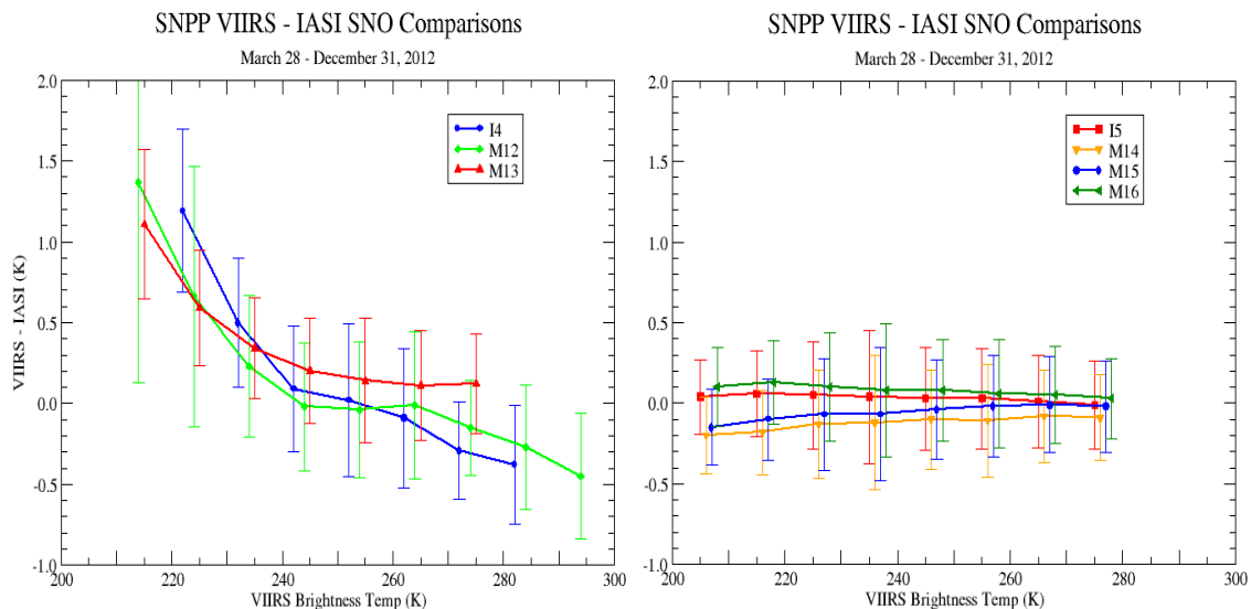
Figure 17.2.3. VIIRS-IASI SNO average differences and standard deviations for MWIR bands (left) and LWIR bands (right). Data points for each band slightly offset on x-axis to declutter. VIIRS MWIR band differences exhibit a pronounced scene temperature dependence that exceeds 1K. VIIRS LWIR band differences suggest a small scene temperature dependence of about 0.2 K in M15, and closer to 0.1K in M14 and M16. Mitigation of this systematic behavior is under review.
