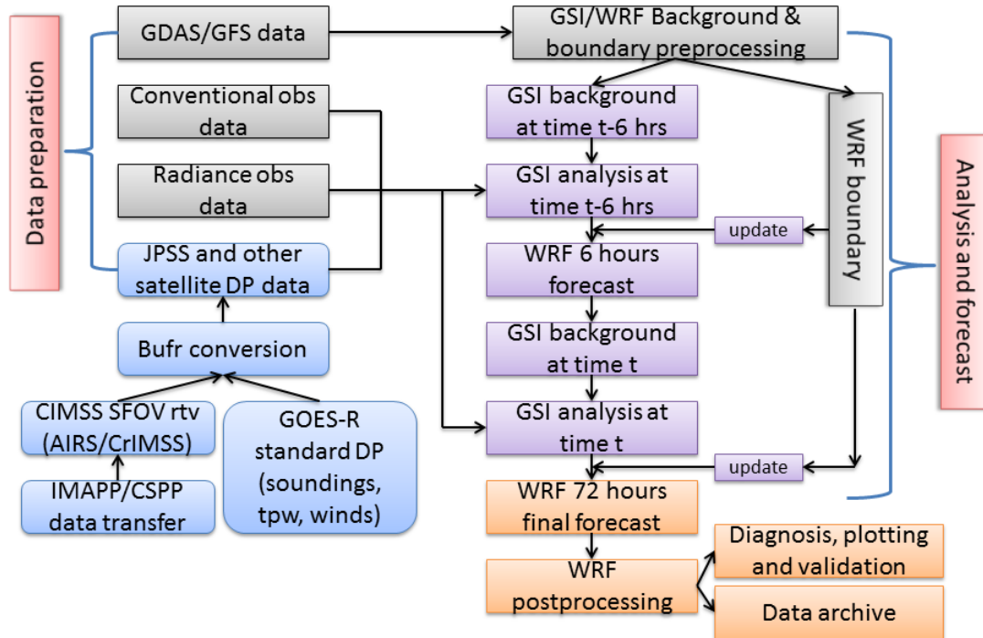
Figure 12.1. Flowchart of GOES-R (legacy soundings, tpw, winds) and JPSS sounding assimilation system for tropical cyclone forecasts.
