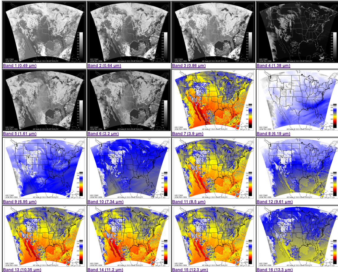
Figure 8.1.1. GOES-R simulated ABI imagery available through our Web site.
