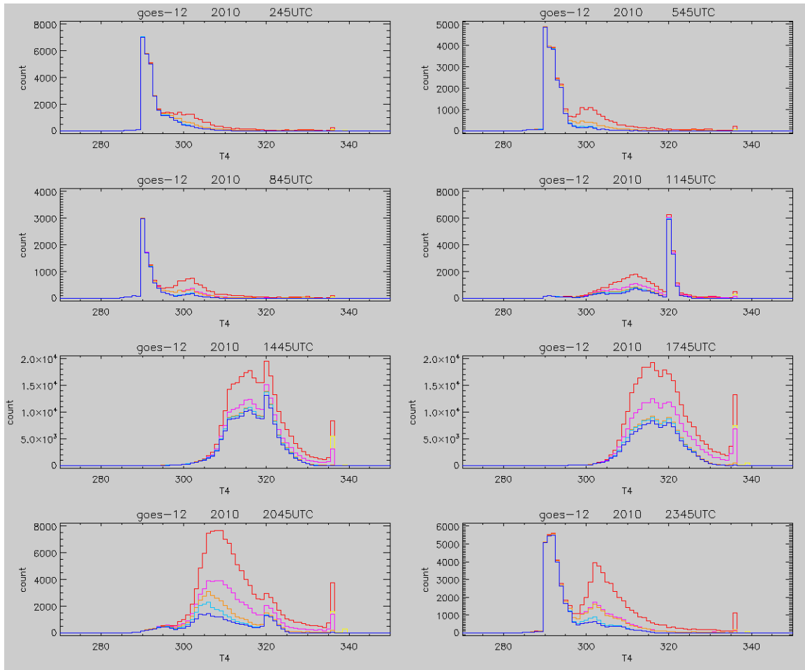
Figure 3.5.2. Histograms of fires binned by observed 3.9 \mu\text{m} brightness temperature, separated by full-disk scan time and category.
