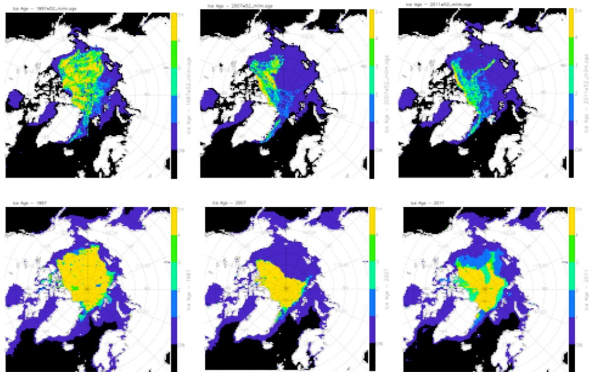
Figure 25.3. Sea ice age for the years of 1987, 2007, and 2011 (Top line from Lagrangian tracking method (CU), bottom line from Eulerian tracking method (UW), both using SSM/I data) in terms of ice age classification (0=open water, 1=first-year ice, 2=second-year ice, 3=third-year ice, 4=fourth-year ice, 5=fifth or more year ice).
