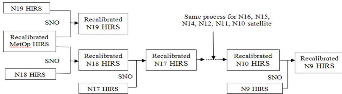
Figure 36.1. Schematic of the recalibration process using Metop IASI and SNOs.
