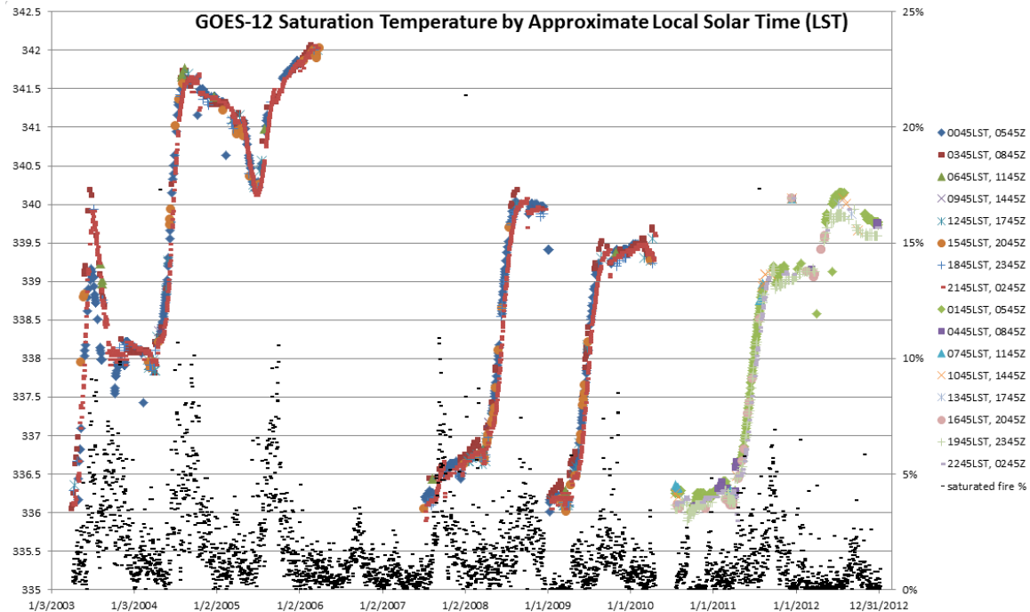
Figure 3.5.1. GOES-12 3.9 \mu\text{m} saturation temperature over time plotted as a function of local solar time. The large shifts caused by onboard contamination of the Imager's optics and subsequent cleanings are clearly visible.
