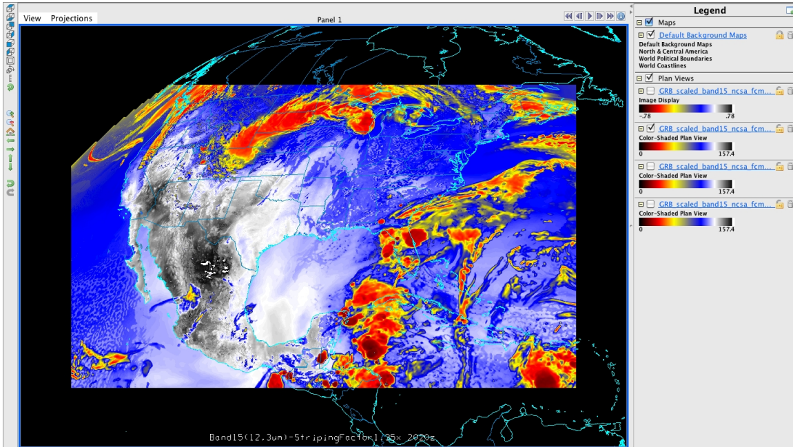
Figure 8.2.1. Simulated ABI band 15 (12.3 micrometer) data for June 4, 2005 at 20:20 UTC with “striping” (increased noise) added every 100 th line. The striping is subtle and not detectable by the naked eye. Displayed in McIDAS-V.
