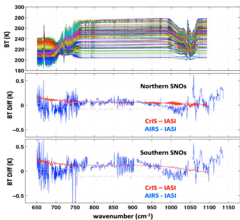
Figure 17.1.1. Summary of on-orbit comparison between CrIS brightness temperature spectra and both AIRS and IASI. All data from February-November 2012 that meets inter-comparison criteria (within 20 minutes, and 3° degrees viewing angle, with viewing angle <30° for AIRS and near nadir for IASI) are used. The dashed curves are error estimates indicating that most of these differences are significant. While these results will be the subject of detailed studies for considerable time, it is clear that the agreement is very good, especially between CrIS and IASI.
