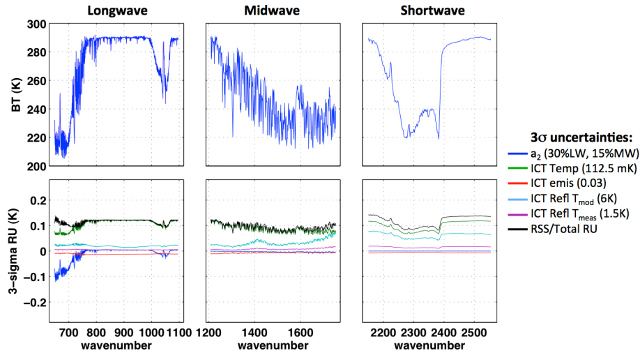
Figure 17.1.2. The Suomi NPP CrIS Radiometric Uncertainty (RU) estimate for a typical Earth view spectrum, with component uncertainties from the nonlinearity corrections ( a_2 uncertainty), ICT temperature uncertainty, ICT emissivity uncertainty, and ICT reflected temperature uncertainty. The RU is less than \sim 0.2 K for all wavenumbers and scene temperatures.
