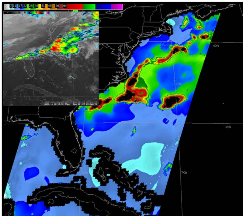
GCOM AMSR-2 Sea-Surface Winds, 0644 UTC 03 December 2018 (Inset: 10.3 μm Clean Window IR Imagery from 0647 UTC)
