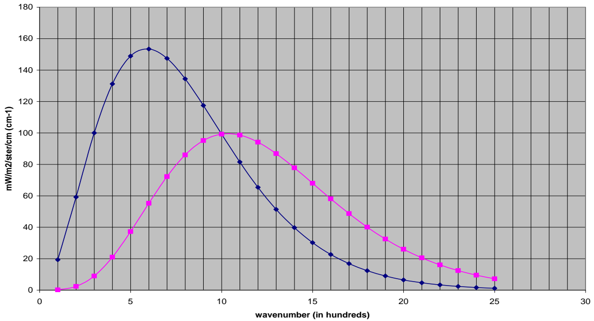
Figure 2.4: Planck radiance curves at 300 K. Wavenumber are given in units of 100 cm -1 ; the corresponding wavelengths in cm are determined from the reciprocal of the wavenumber. Purple boxes show B(\lambda, T) in units of mW/ster/m 2 /cm (per unit wavelength) and blue diamonds show B(\nu, T) in units of mW/ster/m 2 /cm -1 (per unit wavenumber). B(\lambda, T) is shown multiplied by a factor of 10^{-6} (e.g. B(10 \mu\text{m}, 300 \text{ K}) is 9.9 \times 10^7 ) while B(\nu, T) is shown multiplied by a factor of 1 (e.g. B(1000 \text{ cm}^{-1}, 300 \text{ K}) is 99.0). Note that Wiens law for B(\nu, T) becomes \nu(\text{max}) = 1.95T (cm -1 ) while the more familiar form for B(\lambda, T) is \lambda(\text{max}) = .2897/T (cm).
