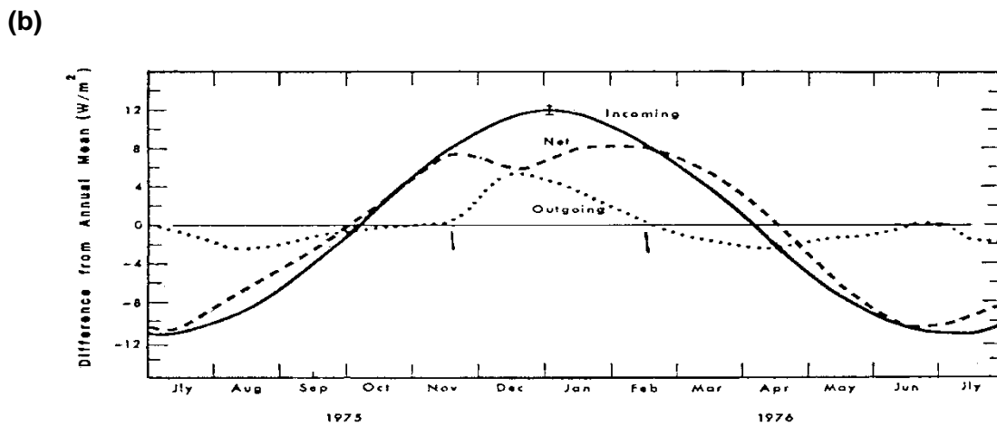
Figure 4.3: (a) Globally averaged monthly mean values of radiation budget parameters. (b) Variation in time with respect to an annual mean of net, incoming, and outgoing radiation.
