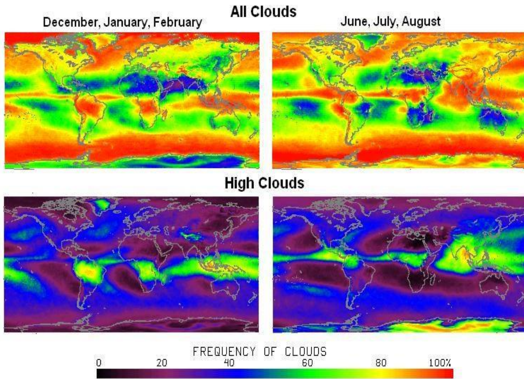
Figure 6.14: The frequency of all clouds and high clouds above 440 hPa from 1979 to 2001 found in HIRS data during winter (December, January, February) and summer (June, July, August).
