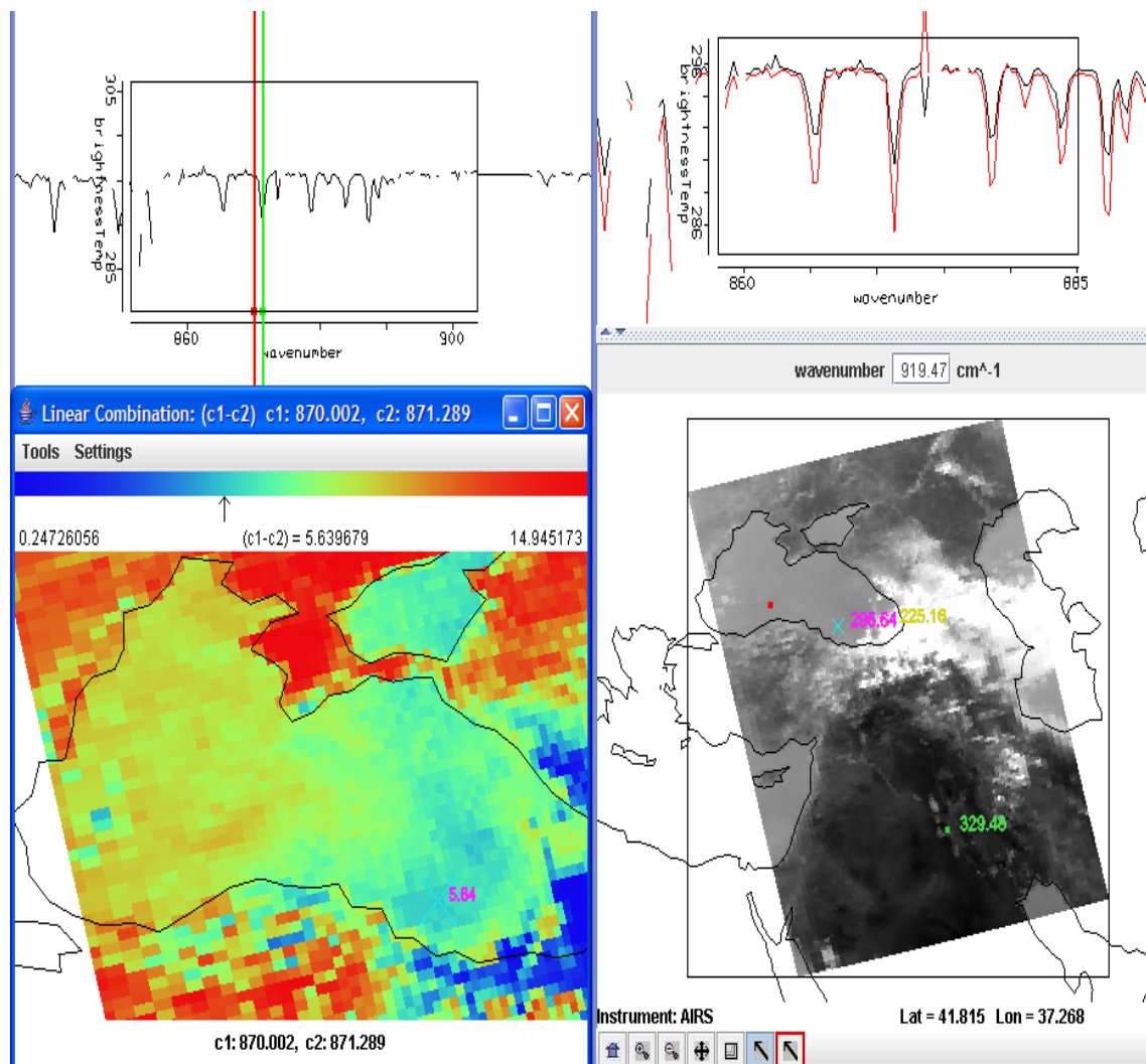
Figure 16.6: (left) Brightness temperature difference of spectral micro-channels at 870.0 \text{cm}^{-1} (off the H 2 O rotational line) minus 871.3 \text{cm}^{-1} (on the H 2 O rotational line). In the western portion of the Black Sea differences are about 9 C while in the eastern portion of the Black Sea they are more like 6 C. There is more low level moisture over the western portion of the Black Sea. (right) The spectra in the window region for the western region (red) show more moisture absorption than the spectra from the eastern region (black).
