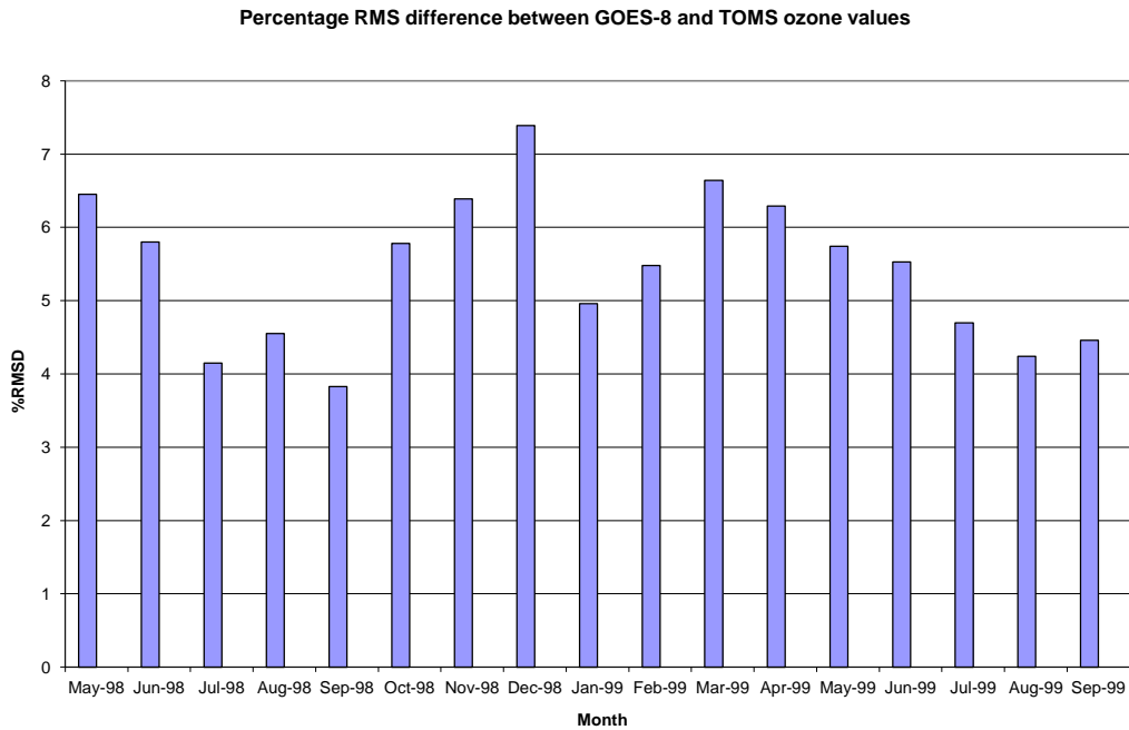
Figure 8.1.a: The monthly % RMSD between the GOES-8 ozone estimates and the TOMS ozone measurements between May 1998 and September 1999.
