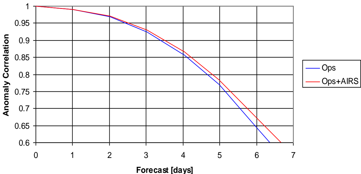
Figure 16.14.b: Anomaly correlation of 500 hPa geopotential heights of the GFS forecasts for January 2004 in the northern hemisphere with and without AIRS data. AIRS adds about 6 hour skill to the five day forecast. From LeMarshall et al (2006).
