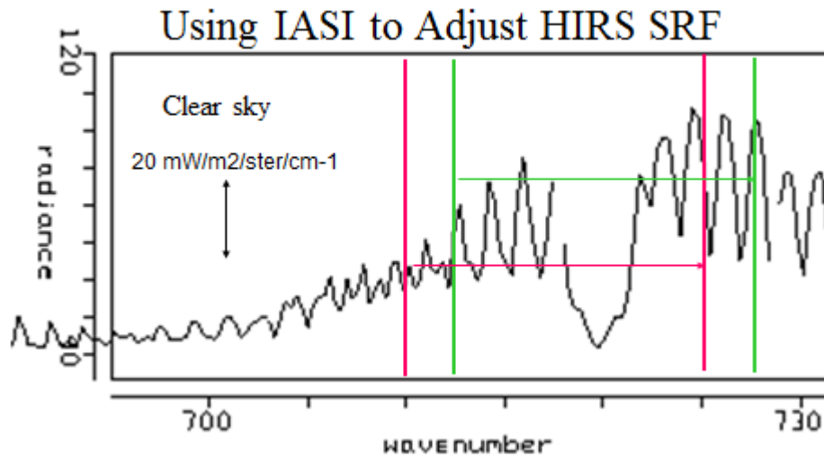
Figure 12.7.c: Using IASI to adjust HIRS Spectral Response Functions (SRFs) illustrated function HIRS band 5 (at 14.0 \mu\text{m} or 715 \text{ cm}^{-1} ). A shift of 2.5 \text{ cm}^{-1} can cause a discrepancy between observed and calculated radiance of about 3 \text{ mW/m}^2/\text{ster/cm}^{-1} (equivalent to a brightness temperature change of about 2 K).
