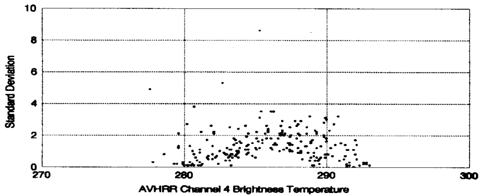
Figure 6.10: Spatial variability test from stratus clouds over South America as an example of the arches obtained for AVHRR 11 \mu m brightness temperatures (x-axis) when plotting local deviation from mean (y-axis).
