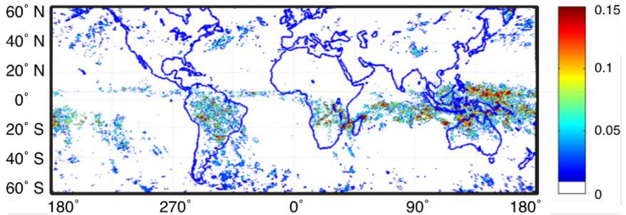
Figure 6.18: Geographical distribution of the fraction of HIRS FOVs indicating the presence of UT/LS clouds for the CO 2 test when BT(14.0 μm) > BT(13.3 μm) using NOAA-14 HIRS data for July 2001.
