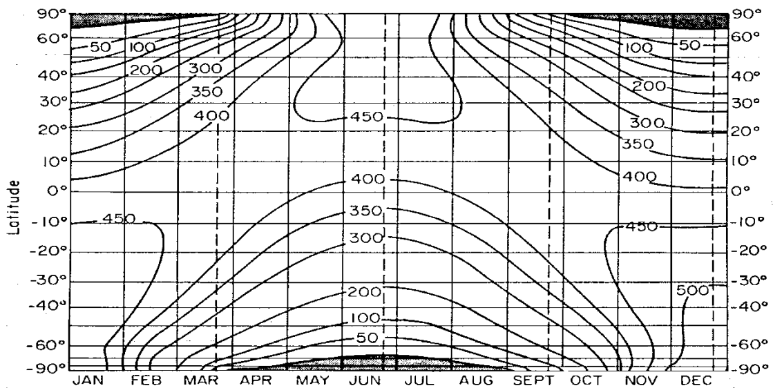
Figure 4.4: Daily solar insolation in \text{W}/\text{m}^2 incident on a horizontal surface at the top of the atmosphere as a function of latitude and date (adapted from Milankovitch, 1930).
