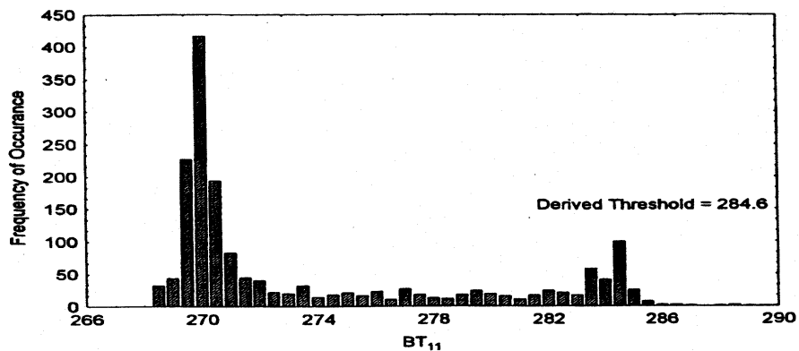
Figure 6.9: Example of infrared histogram analysis technique using AVHRR data for 2.5 by 2.5 degree ocean region. The derived clear sky brightness temperature threshold is 284.6 K.
