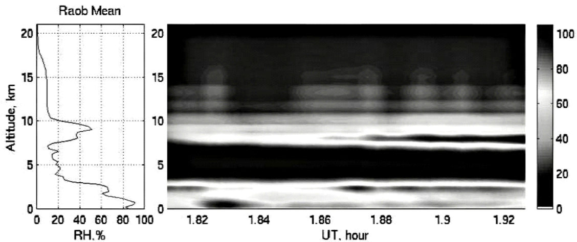
Figure 16.5: Radiosonde (left) shows moist slots in same locations as the infrared interferometer (right) flown during CAMEX-3 on 18 September 1998.
