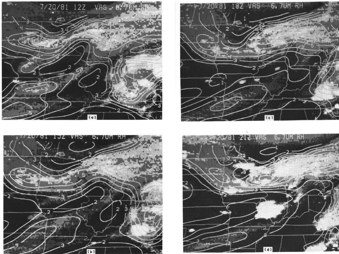
Figure 10.2: Upper tropospheric relative humidity (%/10) superimposed over the VAS image of 6.7 micron atmospheric water vapour radiance emission for (a) 12 GMT, (b) 15 GMT, (c) 18 GMT, and (d) 21 GMT on 20 July 1981.
