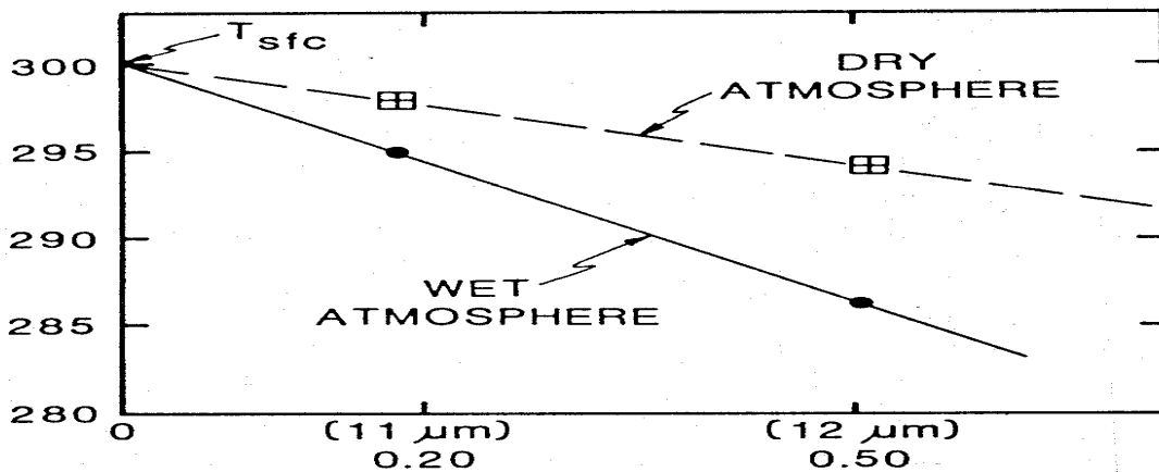
Figure 7.2b: Graphic representation of the linear relation between water vapour attenuation (x-axis) and brightness temperature (y-axis) for two different atmospheric conditions.
