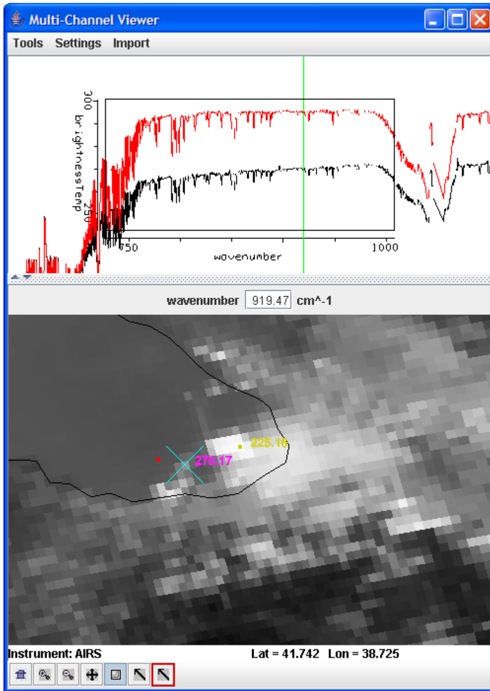
Figure 16.9: Clear sky (red) and thin ice (black) cloud spectra. Between 800 and 1000 \text{cm}^{-1} the brightness temperature of the thin ice cloud spectrum increases with increasing wavenumber. This is caused by the decrease in absorption (hence increase in transmission) of ice from 800 to 1000 \text{cm}^{-1} .
