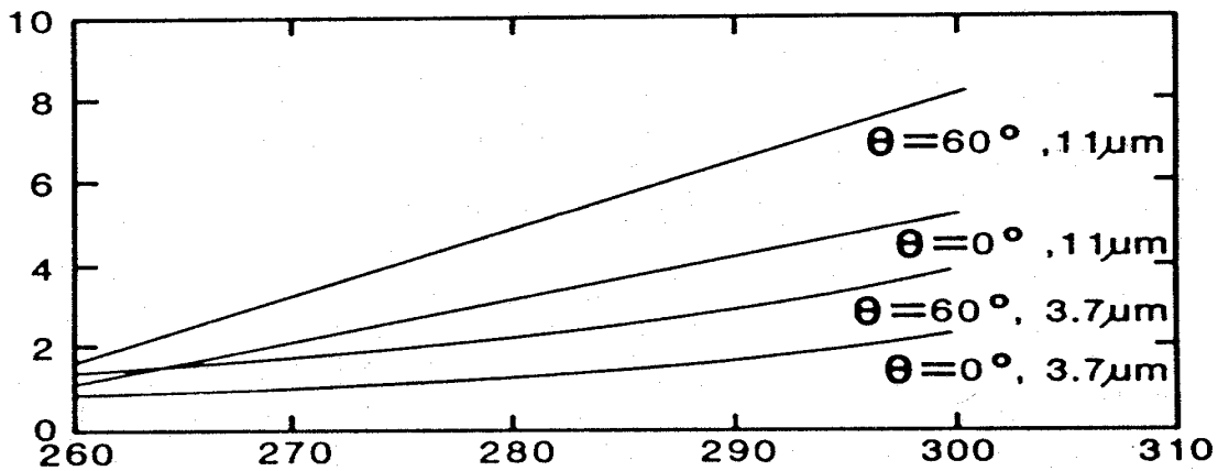
Figure 7.2a: Statistical relations of the water-vapour correction (y-axis) as a function of observed brightness temperature (x-axis) for two spectral channels and two viewing angles.
