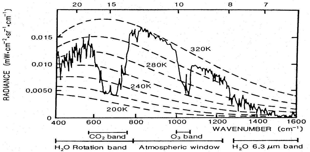
Figure 1.1: Infrared portion of the earth-atmosphere emitted radiation to space observed from Nimbus 4. Planck emission and line spectra are indicated.
