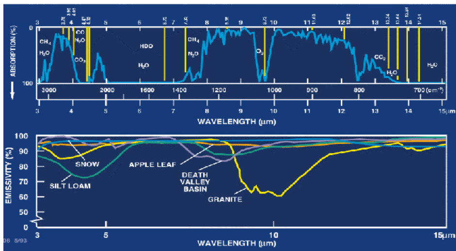
Figure 13.5.d: Atmospheric absorption (top) & surface emissivity (bottom) from 3 to 15 μm.
