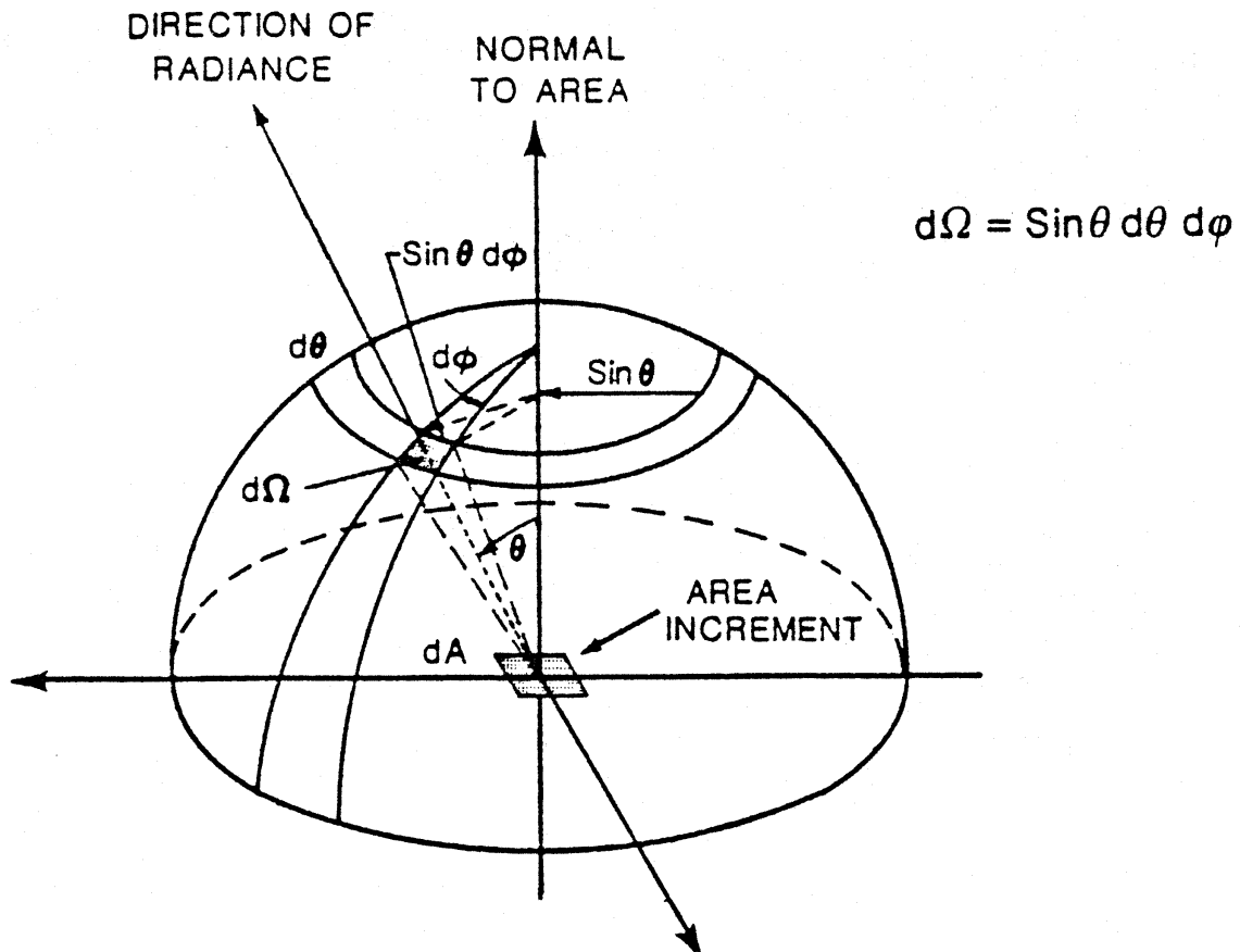
Figure 2.1: The radiance geometry in spherical coordinates
