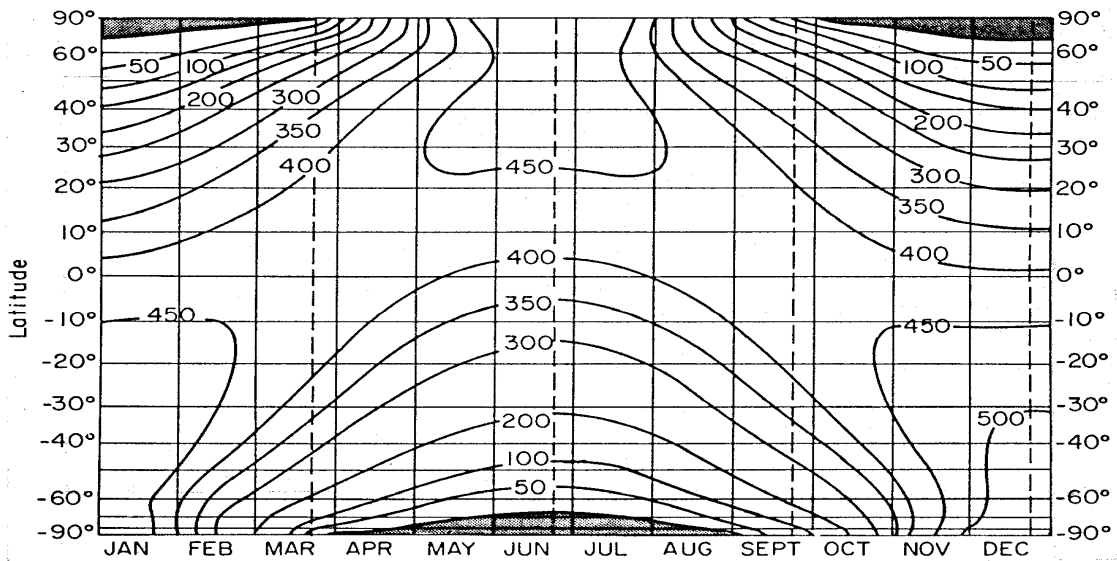
Figure 4.4: Daily solar insolation in W/m^2 incident on a horizontal surface at the top of the atmosphere as a function of latitude and date (adapted from Milankovitch, 1930).
