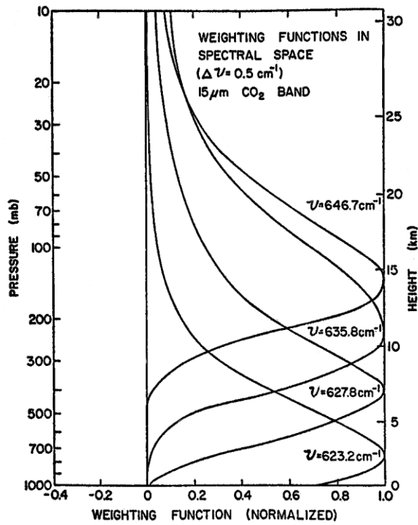
Figure 12.8.c: Spectral radiance temperature profile weighting functions for several frequencies.
