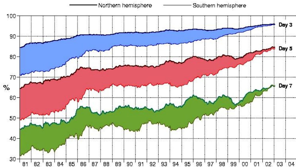
Figure 1.6: 500 hPa anomaly correlation for the European Centre for Medium range Weather Forecast (ECMWF) 3, 5, and 7 day forecasts in the northern and southern hemisphere from 1981 to 2004. Most recently equal forecast skill is evident in both hemispheres, the in-situ data rich northern hemisphere and the in-situ data poor southern hemisphere; improved assimilation of satellite data is making this possible.
