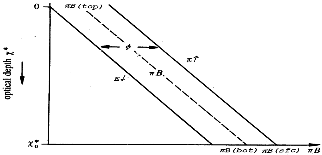
Figure 4.7: Upward E\uparrow and downward E\downarrow irradiance and emitted radiance from a given layer \pi B (given by Stefan's Law) plotted as a function of effective optical depth \chi^* in an atmosphere in radiative equilibrium.
