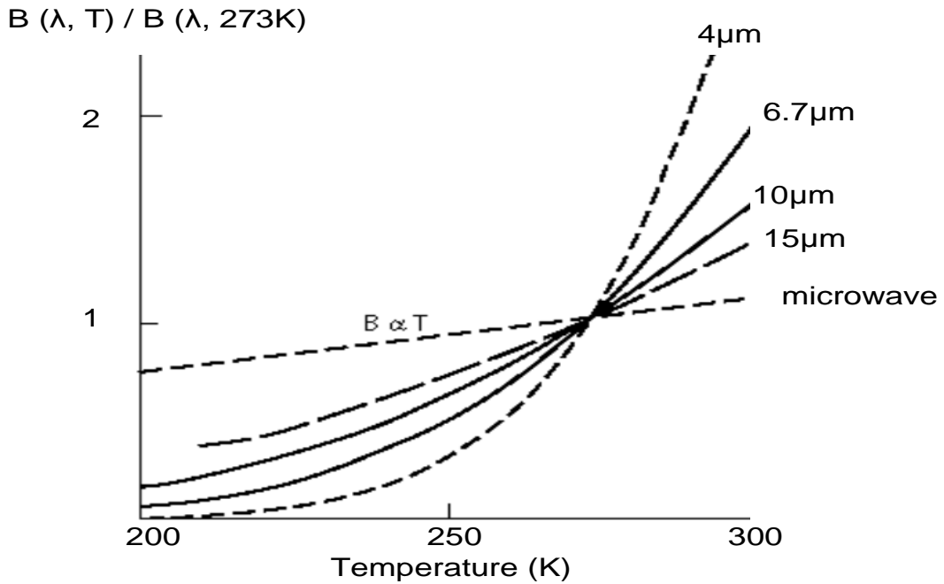
Figure 2.7: Temperature dependence of the Planck function B(\lambda, T) for earth scene temperatures
