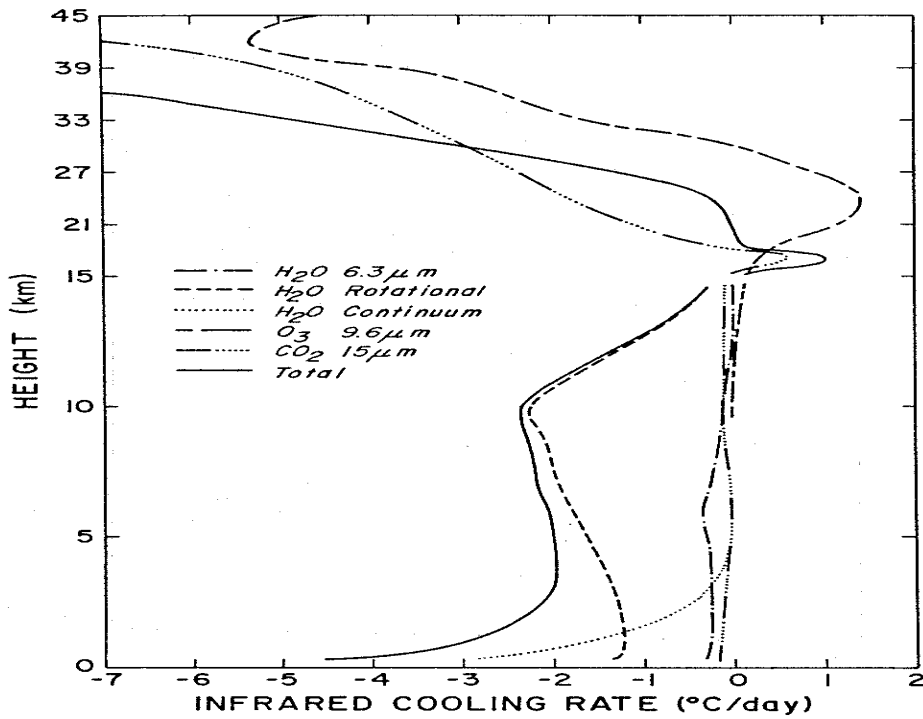
Figure 4.6: Calculation of total and partial cooling rates with an atmospheric profile appropriate for clear tropical conditions (after Roewe and Liou, 1978).
