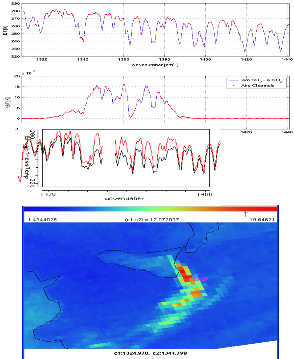
Figure 16.13: The spectral signature of SO 2 between 1320 and 1400 cm -1 (top) offers the opportunity to track volcanic SO 2 emissions. The spectrum for Mt Etna of 28 Oct 2002 (middle) suggests that the brightness temperature difference of 1325 minus 1345 cm -1 (avoiding water vapor absorption lines) effectively maps Volcanic SO 2 emissions.
