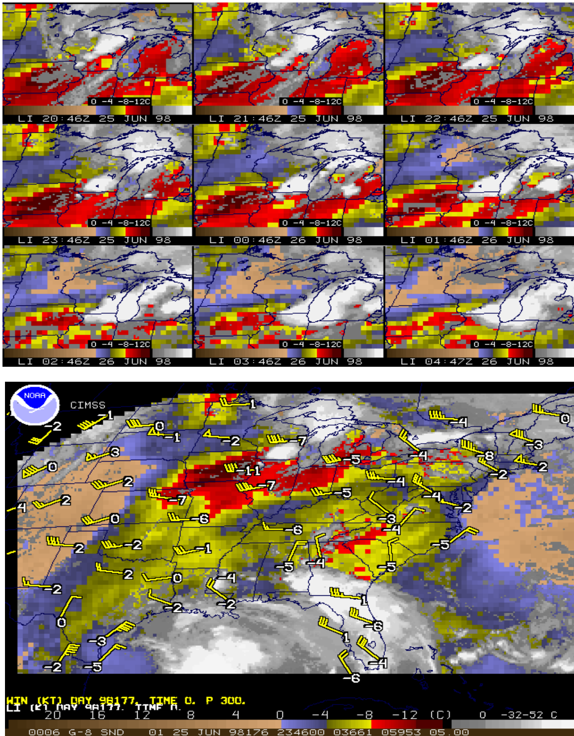
Figure 10.8: (top) GOES DFI of Lifted Index from 2046 to 0446 UTC at 2346 UTC on 25 June 1998 show extreme instability associated with a frontal passage across Minnesota and Wisconsin. (bottom) Radiosonde reports of lifted indices are overlaid on 2346 UTC DFI as are the wind reports.
