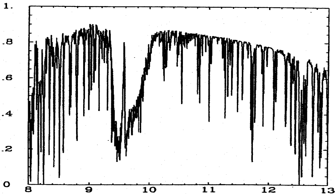
Figure 6.2: High spectral resolution total transmittance spectra for a standard atmosphere from 8 to 13 microns.
