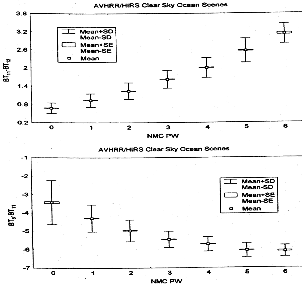
Figure 6.4: The dependence on PW of the brightness temperature difference between the various window channels. Observed AVHRR 11-12 micron (top panel) and collocated HIRS 8-11 micron (bottom panel) brightness temperature differences plotted versus global model (NMC) total column PW for January 1994 over clear ocean scenes.
