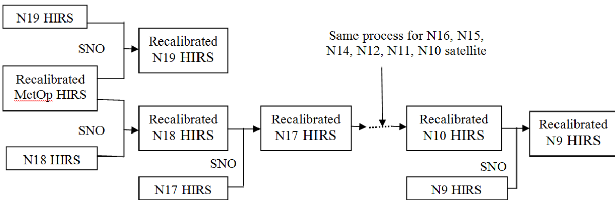
Figure 12.7.b: Inter-satellite calibration process for the HIRS on the NOAA satellite series, using Metop-A HIRS as a reference sensor.
