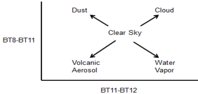
Figure 6.5: Schematic diagram of the effects of different atmospheric constituents on the brightness temperature differences 11 minus 12 microns and 8.6 minus 11 microns.
