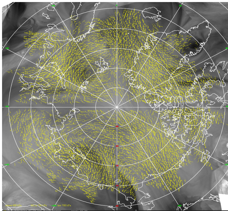
Figure 9.8: Wind vectors derived from infrared cloud and water vapor features of successive MODIS passes over the Arctic. This is the daily coverage of Atmospheric Motion Vectors (AMVs) from Terra overlaid on a daily water vapor image composite.
