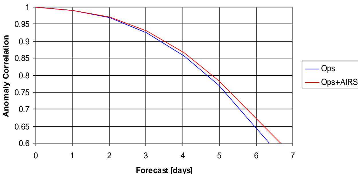
Figure 16.14.b: Anomaly correlation of 500 hPa geopotential heights of the GFS forecasts for January 2004 in the northern hemisphere with and without AIRS data. AIRS adds about 6 hour skill to the five day forecast. From LeMarshall et al (2006).
