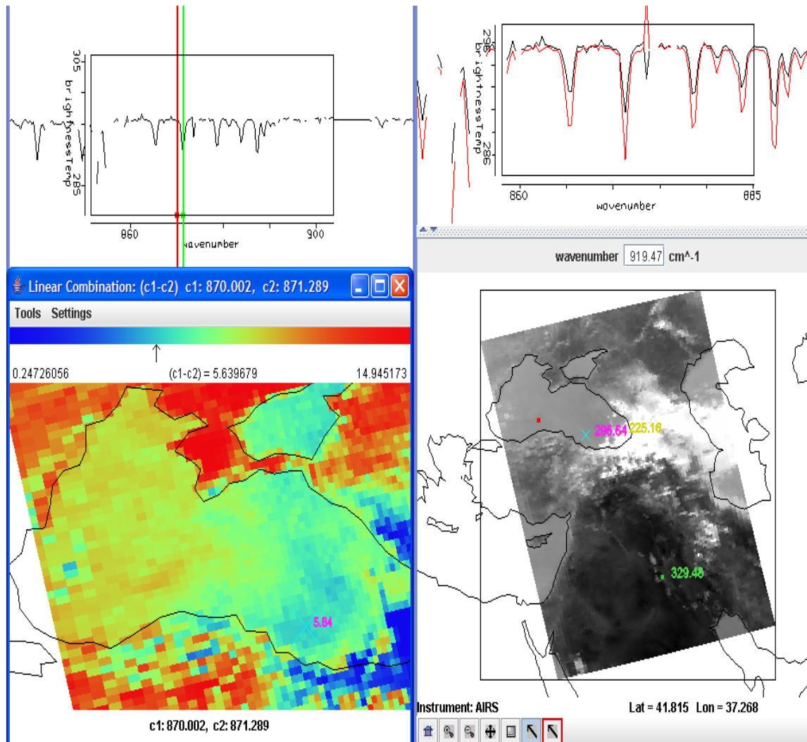
Figure 16.6: (left) Brightness temperature difference of spectral micro-channels at 870.0 \text{cm}^{-1} (off the H 2 O rotational line) minus 871.3 \text{cm}^{-1} (on the H 2 O rotational line). In the western portion of the Black Sea differences are about 9 C while in the eastern portion of the Black Sea they are more like 6 C. There is more low level moisture over the western portion of the Black Sea. (right) The spectra in the window region for the western region (red) show more moisture absorption than the spectra from the eastern region (black).
