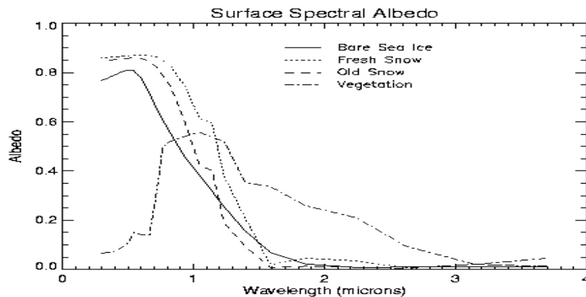
Figure 6.8: Albedo variations for ice, snow, and vegetation from 0.5 to 3.5 microns. Vegetation shows a sharp increase above 0.72 microns. Snow/ice shows a sharp decrease above 1.4 microns.
