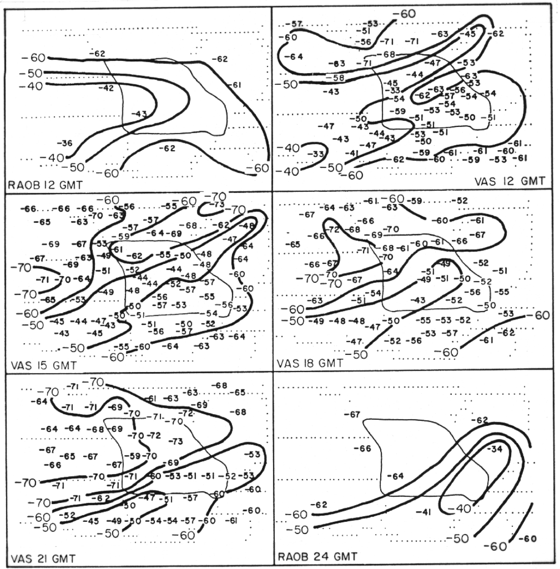
Figure 10.5: Radiosonde and VAS observations of 300 hPa dewpoint temperature (degrees Centigrade) on 20 July 1981.
