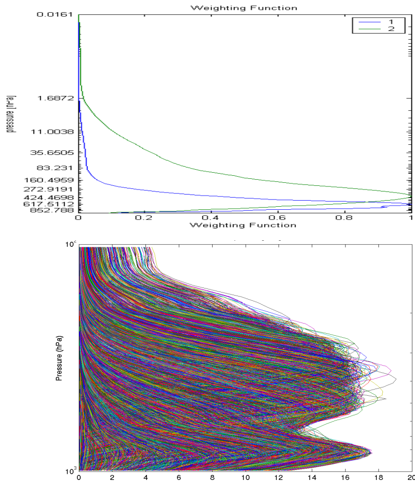
Figure 16.4: (top) Weighting functions for off-line (peaking at 600 hPa) and on-line (peaking at 400 hPa) measurements at 735 cm -1 . (bottom) The weighting functions associated with roughly 3000 high spectral IR resolution micro-channels for a standard atmosphere.
