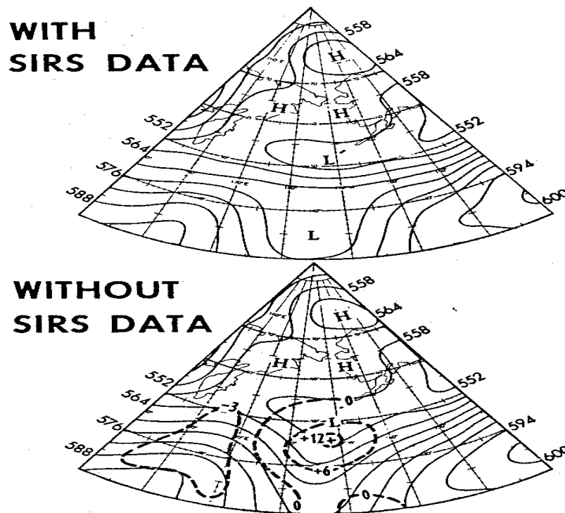
Figure 1.2: Comparison of objective analyses of 500 mb height for 24 June 1969 obtained with and without SIRS soundings. The differences in decameters are shown by the dashed isolines. Note the difference over the Pacific where the SIRS data indicate a cut-off low with an intense jet to the north instead of a diffusely defined trough. Extended range (72 hr) forecasts for North America displayed maximum errors based on the analyses with SIRS of only half the magnitude of those resulting without the use of the data.
