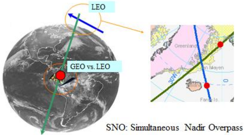
Figure 12.7.a: Illustration of Inter-satellite Calibration of LEO and GEO using the Simultaneous Nadir Overpass (SNO) Method.
