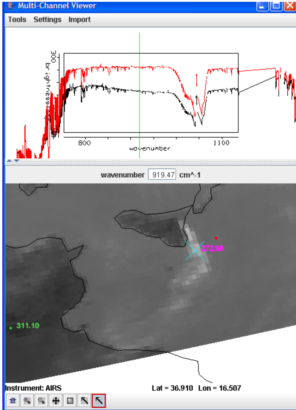
Figure 16.12: Clear sky (red) and Mt Etna volcanic ash (black) spectra for 28 October 2002. Between 800 and 1000 cm -1 the brightness temperature of the volcanic ash spectrum decreases with increasing wavenumber. This is caused by the increase in absorption (hence decrease in transmission) of ash from 800 to 1000 cm -1 . Between 1080 and 1120 cm -1 the opposite occurs.
