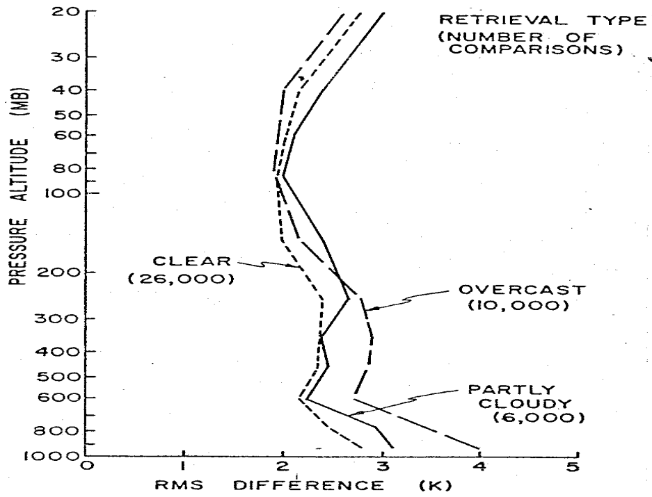
Figure 1.3: RMS differences between radiosonde and satellite temperature soundings for April 1980.
