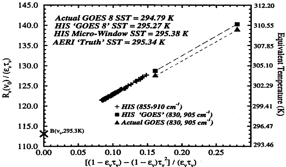
Figure 7.5: HIS and GOES radiance observations plotted in accordance with the radiative transfer equation including corrections for atmospheric moisture, non-unit emissivity of the sea surface, and reflection of the atmospheric radiance from the sea surface. Radiances are referenced to 880 cm -1 . The intercept of the linear relationship for each data set represents a retrieved surface skin blackbody radiance from which the SST can be retrieved.
