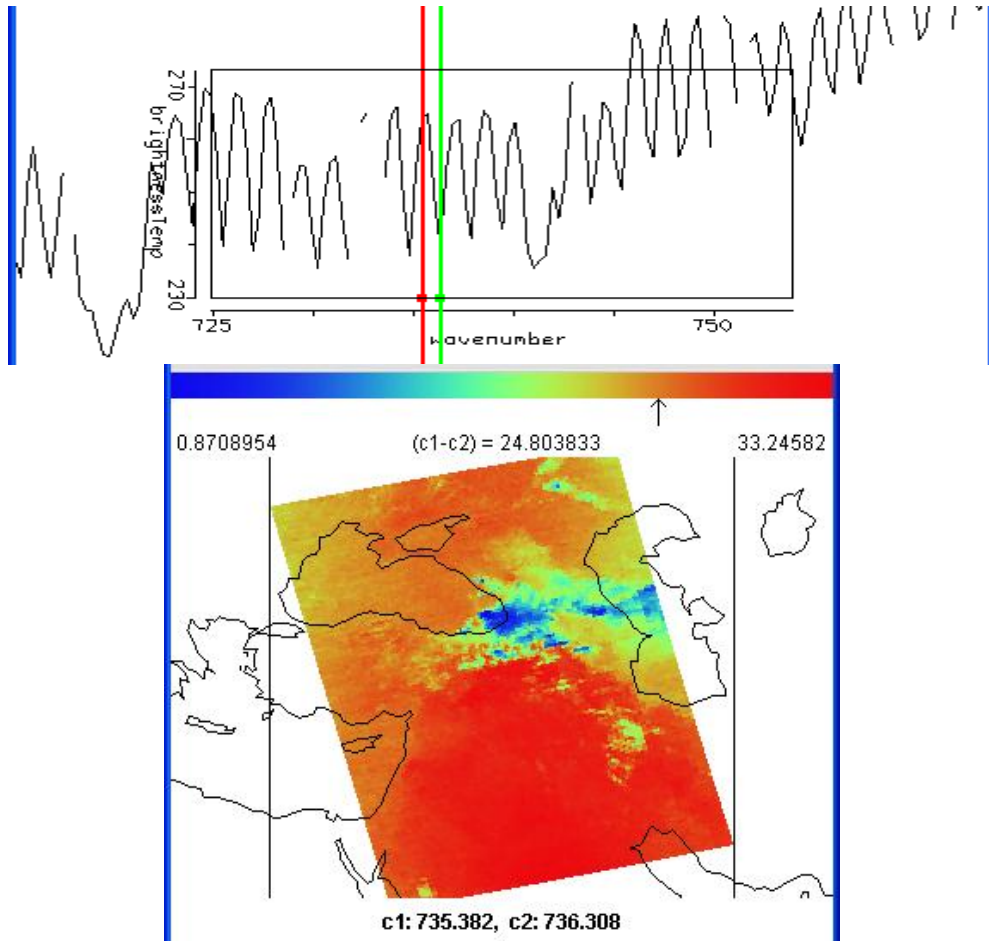
Figure 16.3: Brightness temperature difference of spectral micro-channels at 735.4 \text{cm}^{-1} (off the \text{CO}_2 rotational line) minus 736.3 \text{cm}^{-1} (on the \text{CO}_2 rotational line). In clear skies this is as large as 33 C; in high clouds (where little \text{CO}_2 resides above) the difference is small.
