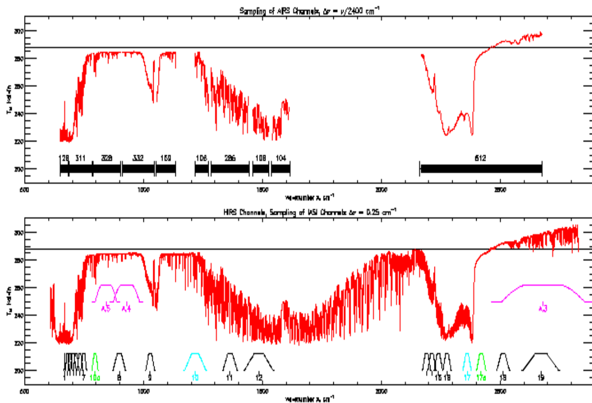
Figure 16.1: Spectral Coverage of AIRS with 2378 micro-channels (top) and IASI with 8461 micro-channels (bottom). Also indicated are the infrared spectral bands of AVHRR and HIRS.
